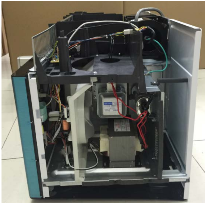
EUT Uncovered View
