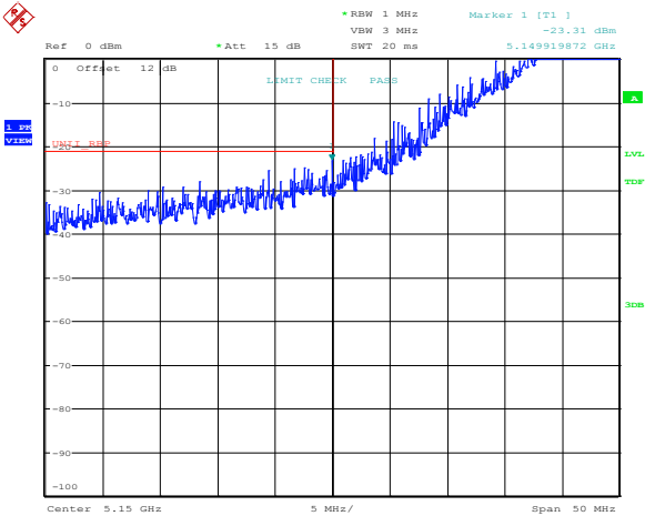
Figure 8.8-149: Lower band edge emission at 5150 MHz, channel 38, 802.11n HT40, cho, Peak
