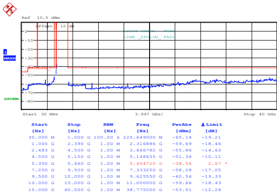
Figure 8.8-97: Spurious emissions within restricted bands at channel 64, 802.11a, ch1
