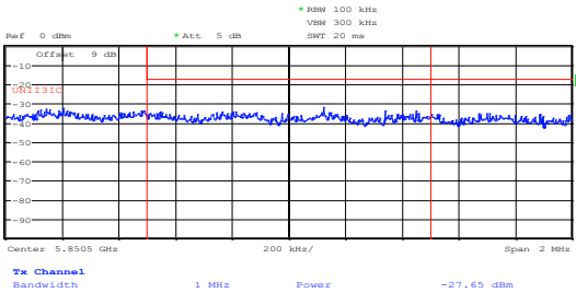
Figure 8.8-170: Upper band edge emission at 5850 MHz, channel 165, 802.11n HT20, cho
