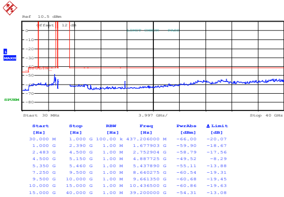
Figure 8.8-85: Spurious emissions within restricted bands at channel 38, 802.11n HT40, ch1
