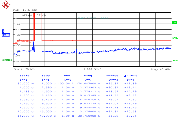
Figure 8.8-77: Spurious emissions within restricted bands at channel 54, 802.11n HT40, cho
