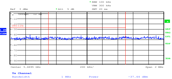
Figure 8.8-166: Lower band edge emission at 5470 MHz, channel 100, 802.11a, ch1
