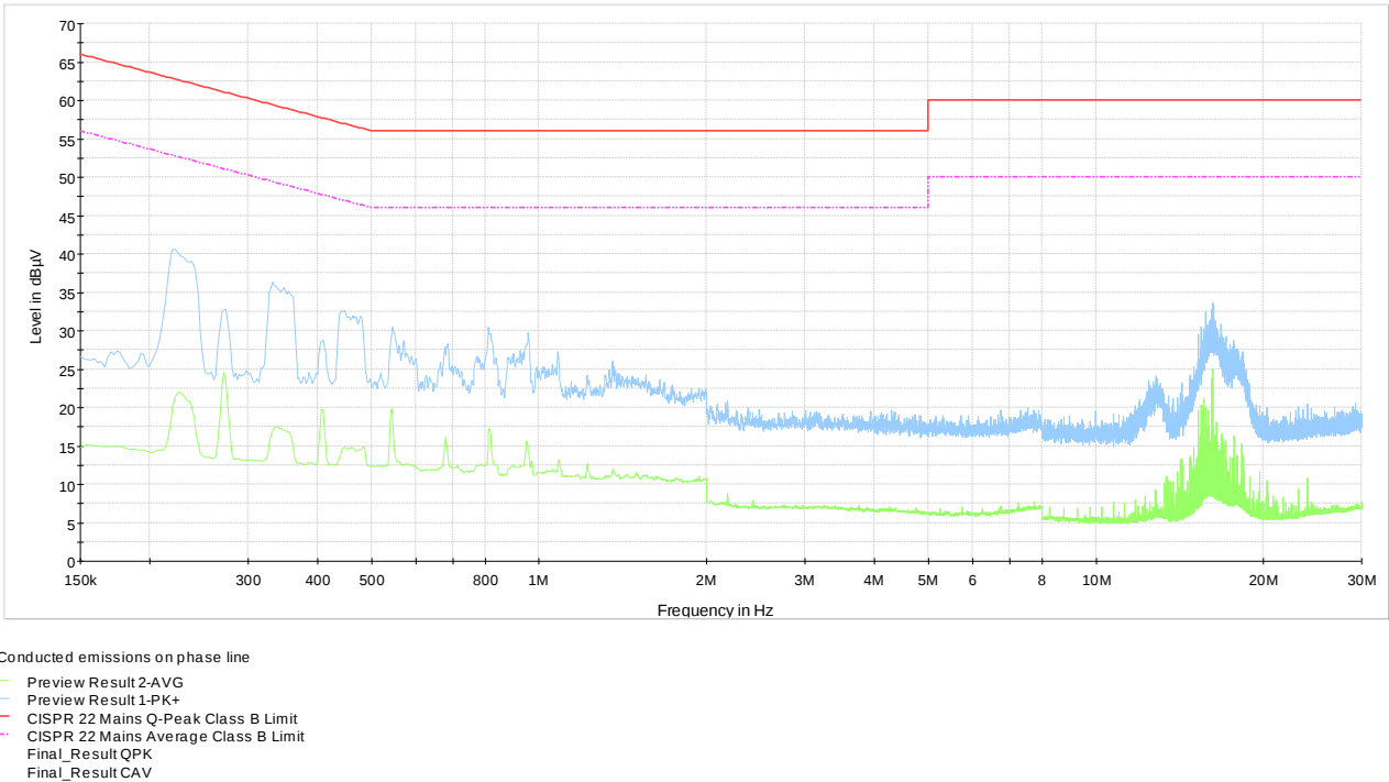
Plot 8.9-5: Conducted emissions on phase line, AC PS
