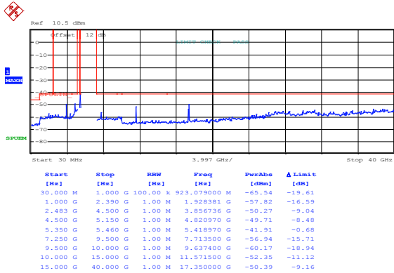
Figure 8.8-109: Spurious emissions within restricted bands at channel 149, 802.11n HT20, cho
