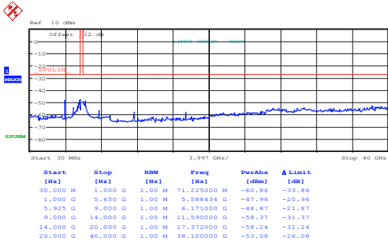
Figure 8.8-45: Spurious emissions outside restricted bands at channel 157, 802.11a, cho
