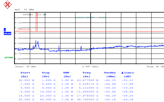
Figure 8.8-46: Spurious emissions outside restricted bands at channel 157, 802.11n HT20, cho
