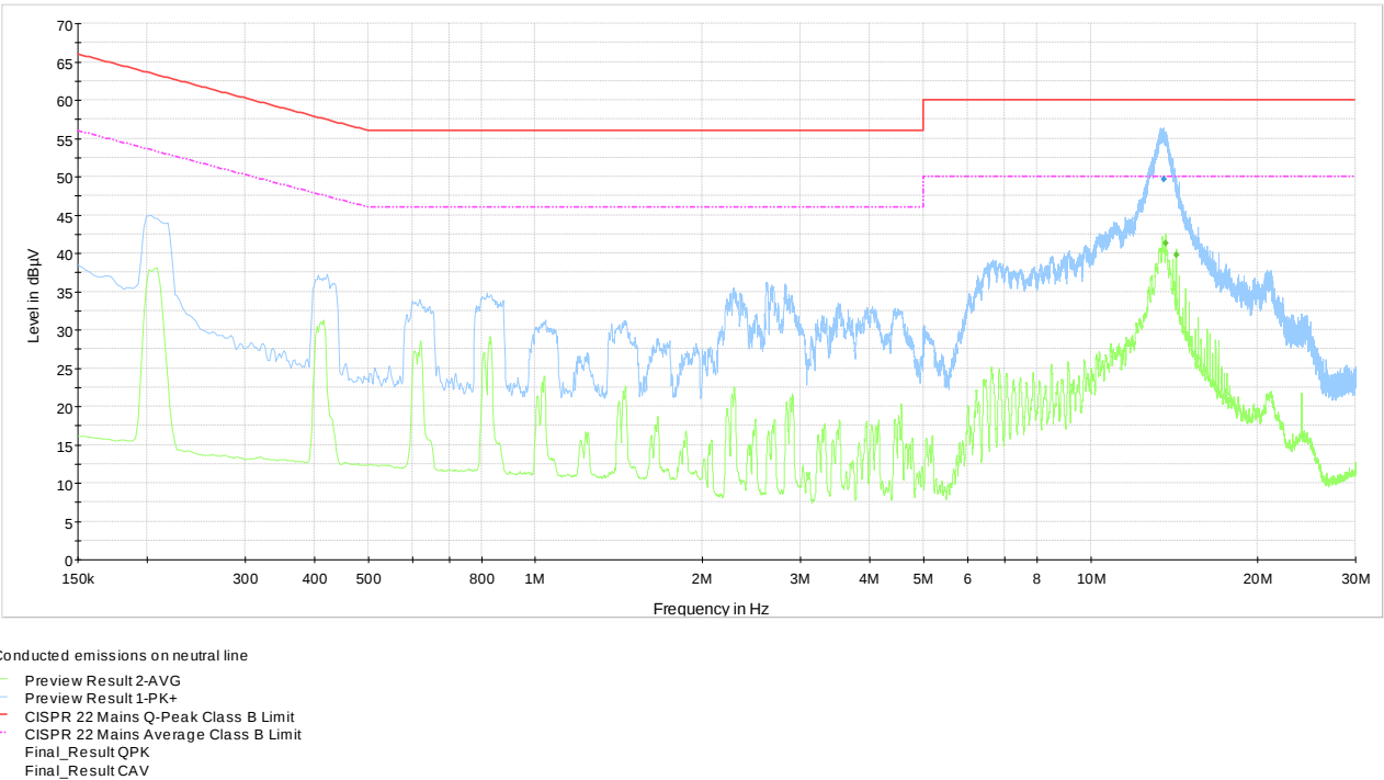
Plot 8.9-2: Conducted emissions on neutral line, 24 V DC PS
