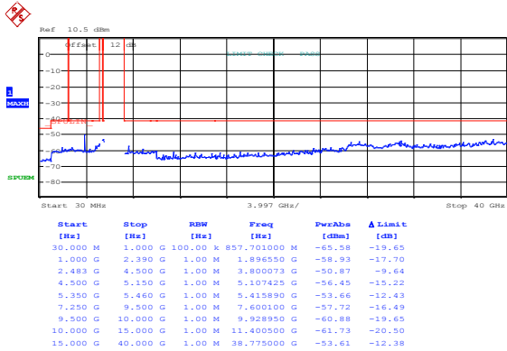
Figure 8.8-105: Spurious emissions within restricted bands at channel 134, 802.11n HT40, cho
