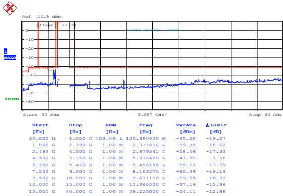
Figure 8.8-65: Spurious emissions outside restricted bands at channel 165, 802.11a, ch1
