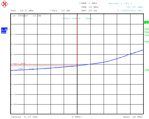
Figure 8.8-146: Lower band edge emission at 5150 MHz, channel 36, 802.11a, cho, Average
