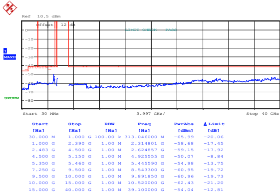
Figure 8.8-89: Spurious emissions within restricted bands at channel 48, 802.11a, ch1
