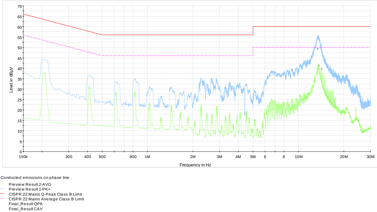
Plot 8.9-1: Conducted emissions on phase line, 24 V DC PS
