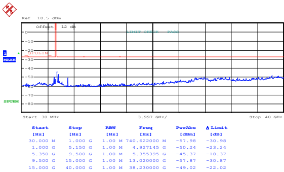
Figure 8.8-25: Spurious emissions outside restricted bands at channel 52, 802.11a, ch1
