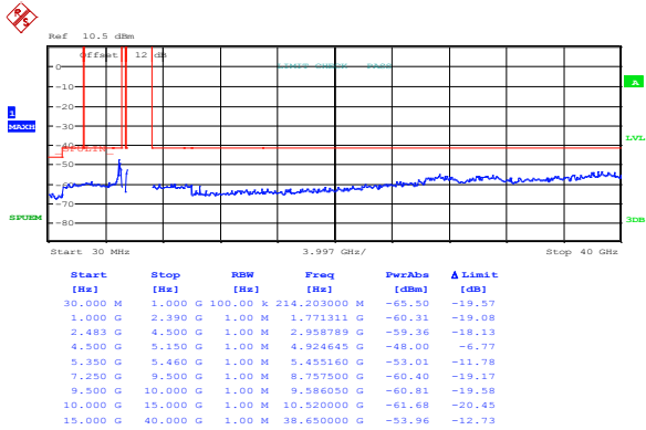
Figure 8.8-73: Spurious emissions within restricted bands at channel 48, 802.11a, cho
