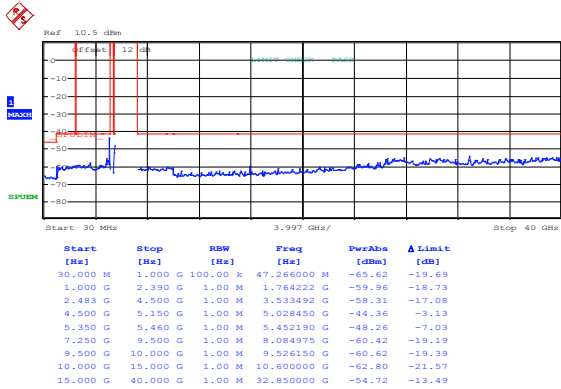
Figure 8.8-93: Spurious emissions within restricted bands at channel 54, 802.11n HT40, ch1
