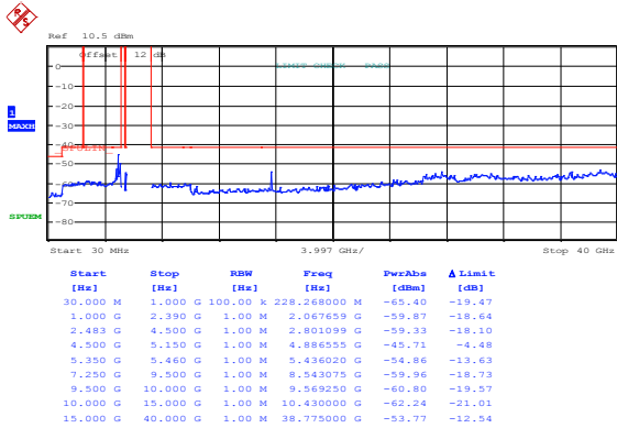
Figure 8.8-69: Spurious emissions within restricted bands at channel 38, 802.11n HT40, cho
