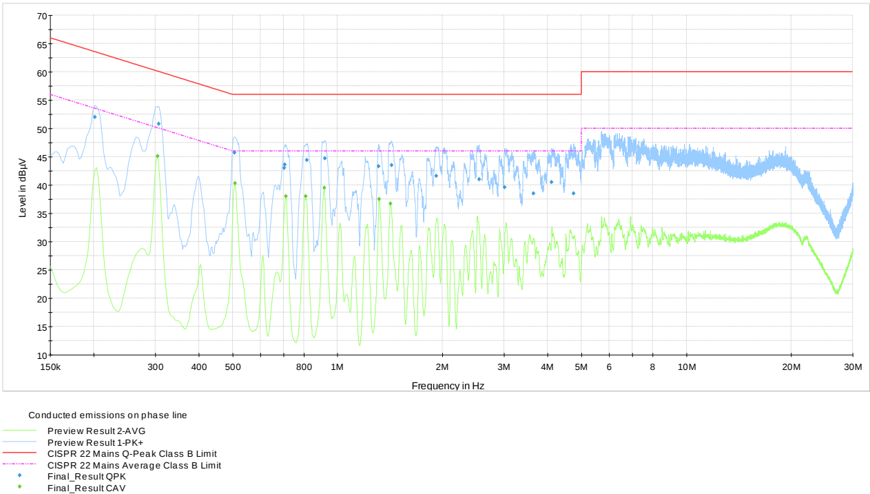
Plot 8.9-3: Conducted emissions on phase line, 48 V DC PS
