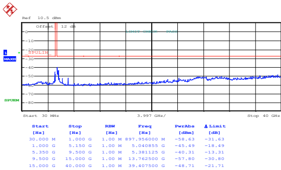
Figure 8.8-26: Spurious emissions outside restricted bands at channel 52, 802.11n HT20, ch1
