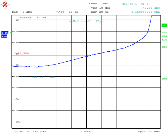
Figure 8.8-154: Lower band edge emission at 5150 MHz, channel 36, 802.11n HT20, ch1, Average
