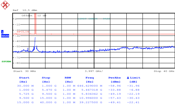
Figure 8.8-49: Spurious emissions outside restricted bands at channel 165, 802.11n HT20, cho
