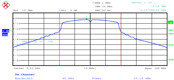
Figure 8.4-1: Sample plot for power and PSD on 802.11a
