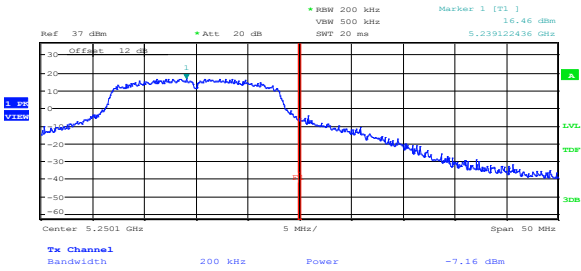
Figure 8.8-185: Upper band edge emission at 5250 MHz (ISED only), channel 46, 802.11n HT40, cho – reference fundamental
