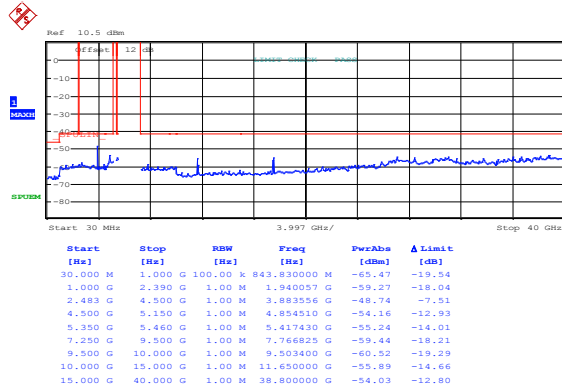
Figure 8.8-113: Spurious emissions within restricted bands at channel 159, 802.11n HT40, cho
