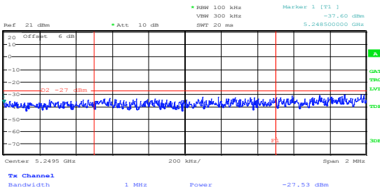
Figure 8.8-158: Lower band edge emission at 5250 MHz, channel 52, 802.11n HT20, cho, ISED only
