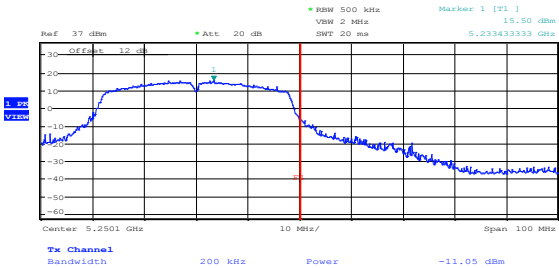
Figure 8.8-189: Upper band edge emission at 5250 MHz (ISED only), channel 48, 802.11n HT20, ch1 – reference fundamental
