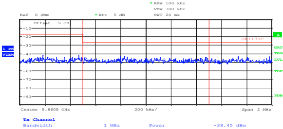
Figure 8.8-177: Upper band edge emission at 5860 MHz, channel 159, 802.11n HT40, cho
