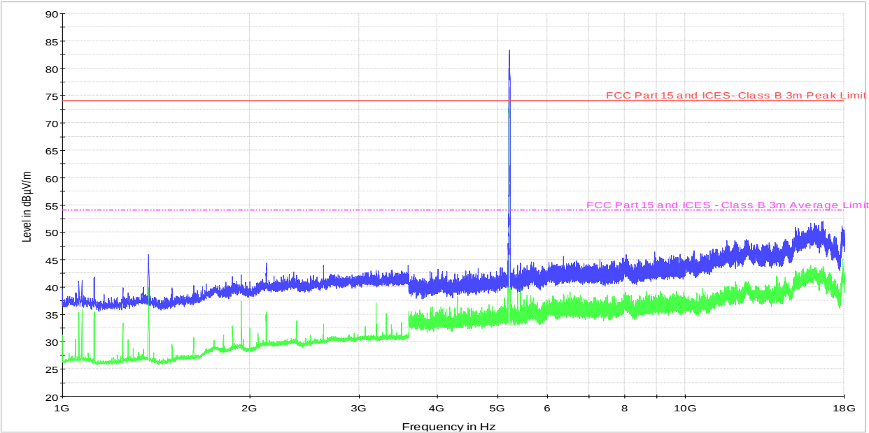
Figure 8.8-211: Spurios radiation outside restricted bands sample plot, 5150–5250 GHz
