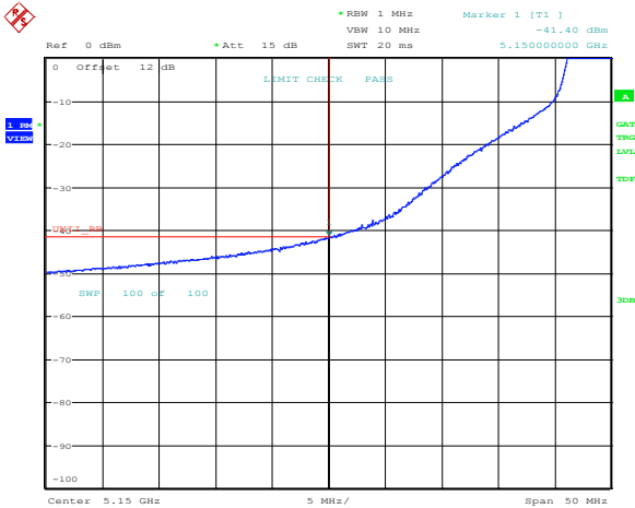
Figure 8.8-150: Lower band edge emission at 5150 MHz, channel 38, 802.11n HT40, cho, Average
