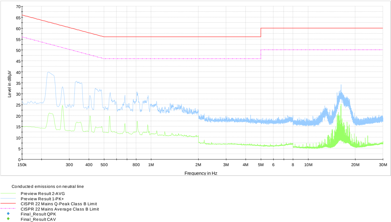
Plot 8.9-6: Conducted emissions on neutral line, AC PS
