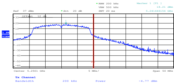
Figure 8.8-181: Upper band edge emission at 5250 MHz (ISED only), channel 48, 802.11a, cho – reference fundamental
