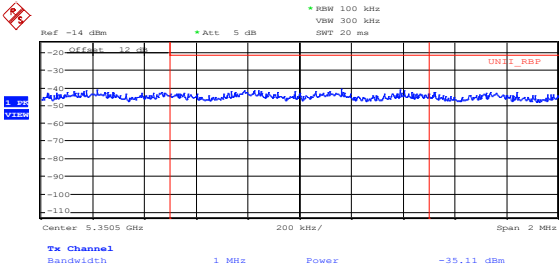
Figure 8.8-201: Upper band edge emission at 5350 MHz, channel 64, 802.11n HT20, ch1, Peak
