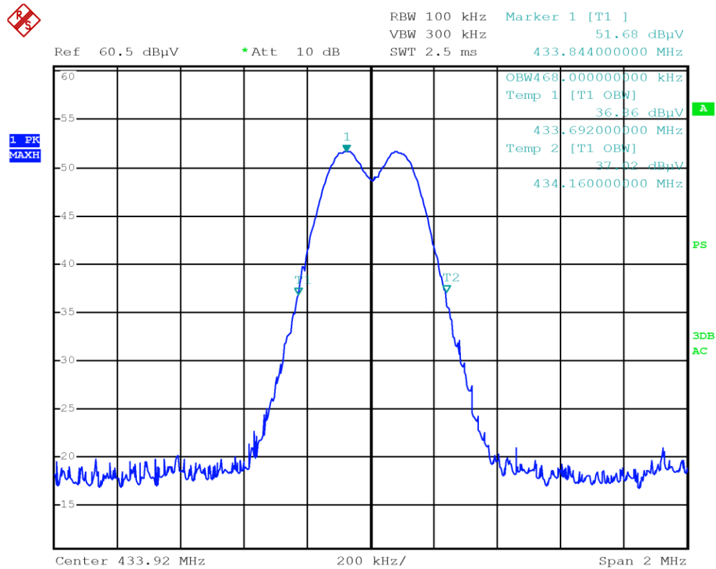
Figure 8.5-2: Occupied bandwidth measurement 99%= 468 kHz
