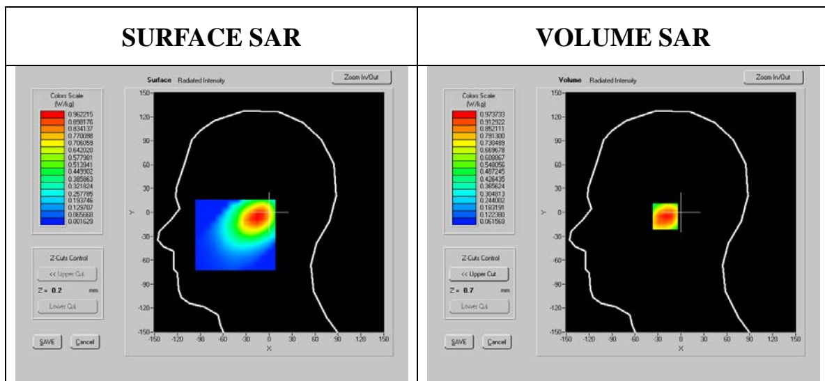
SAR, Z Axis Scan (X = -29, Y = -14)
