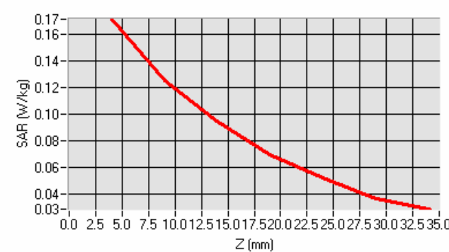
SAR, Z Axis Scan (X = -24, Y = -9)
