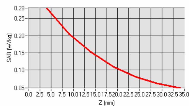
SAR, Z Axis Scan (X = -32, Y = -16)
