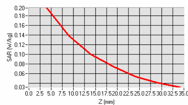
SAR, Z Axis Scan (X = -23, Y = -14)
