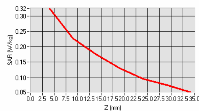
SAR, Z Axis Scan (X = -26, Y = -16)
