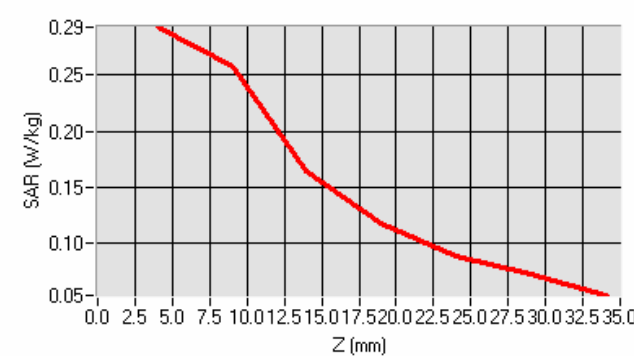
SAR, Z Axis Scan (X = -33, Y = -16)
