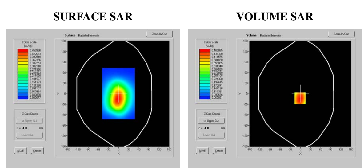
SAR, Z Axis Scan (X = -1, Y = -13)
