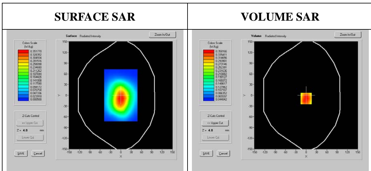
SAR, Z Axis Scan (X = 0, Y = -9)
