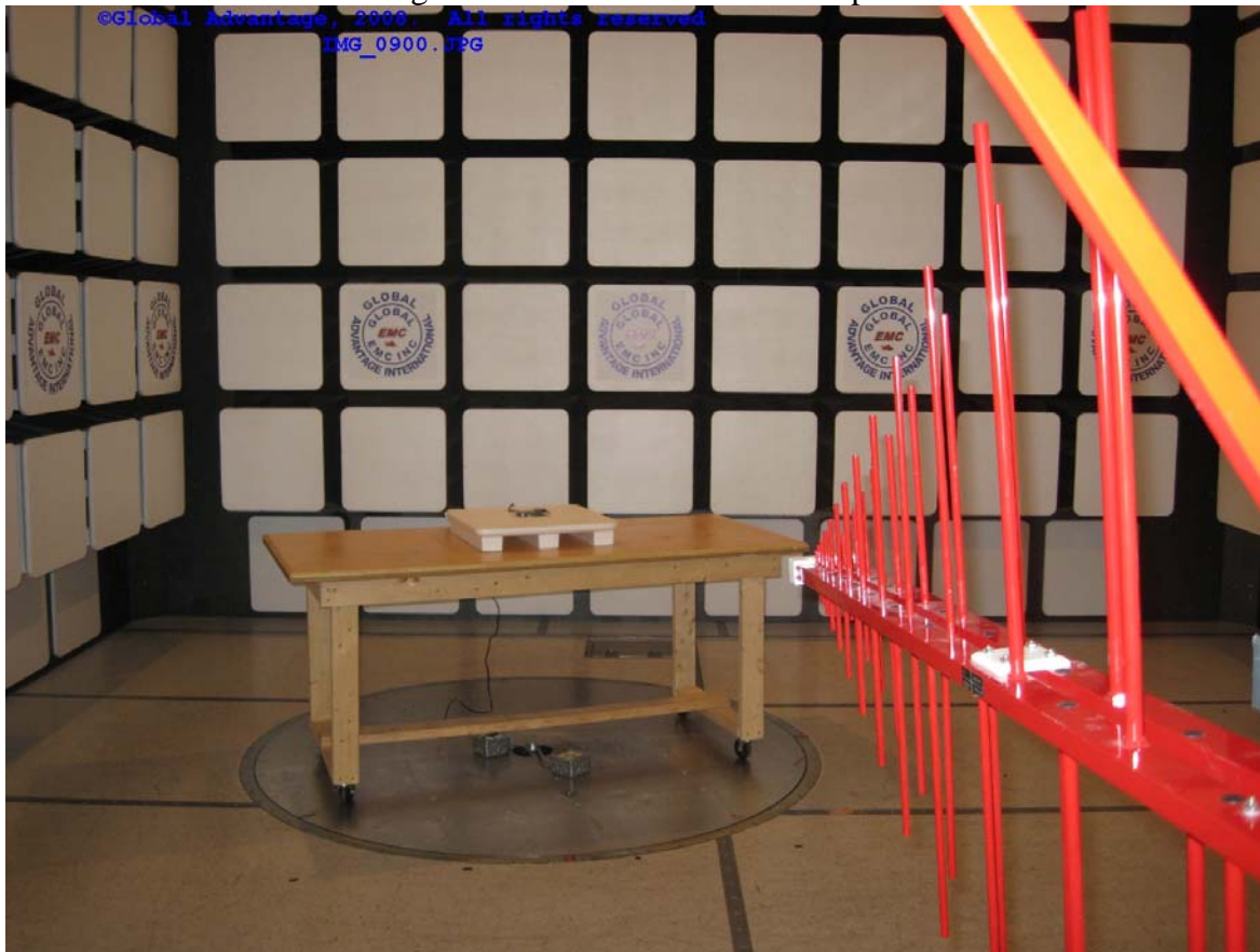
Figure 3 – Radiated emission setup 1
