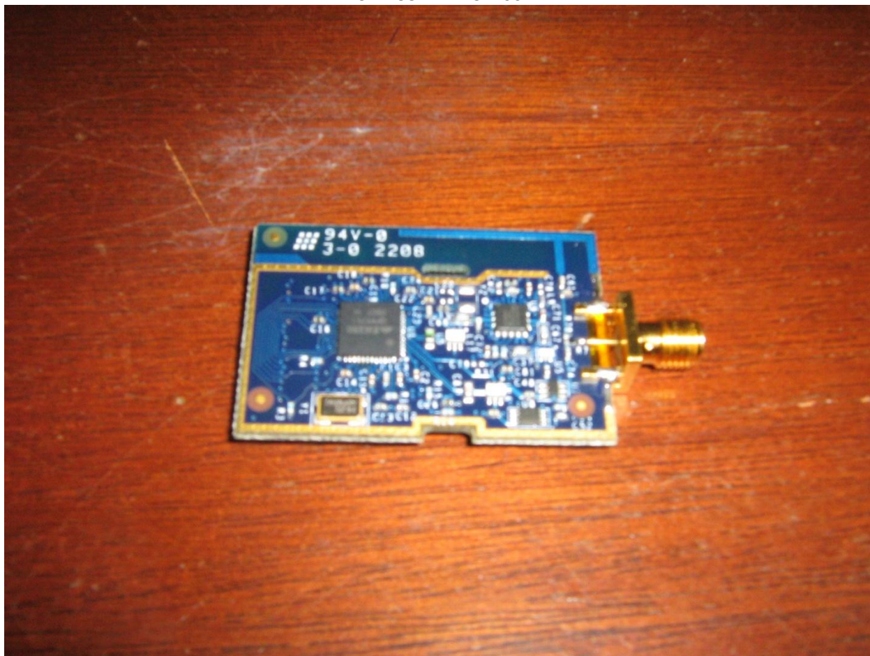
Figure 3 – SMA connector used for conducted emissions testing.
