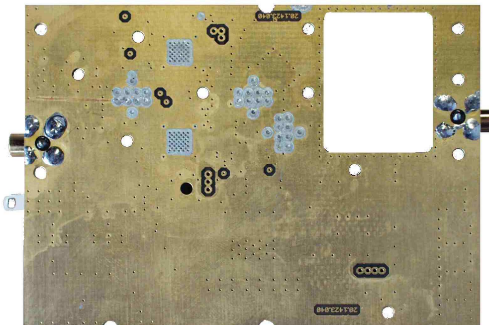
Bottom view
