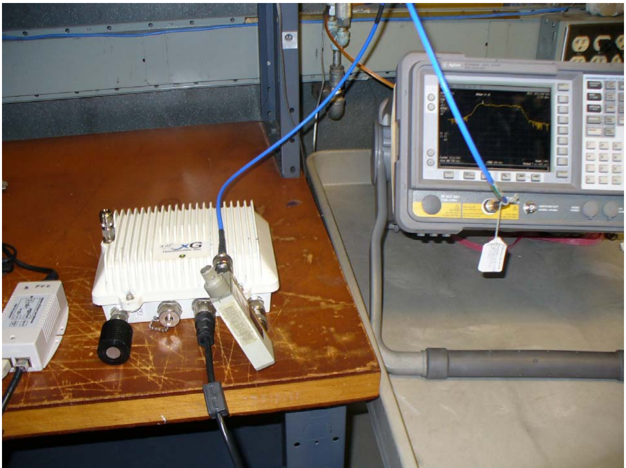
Figure 3: RF Conducted
