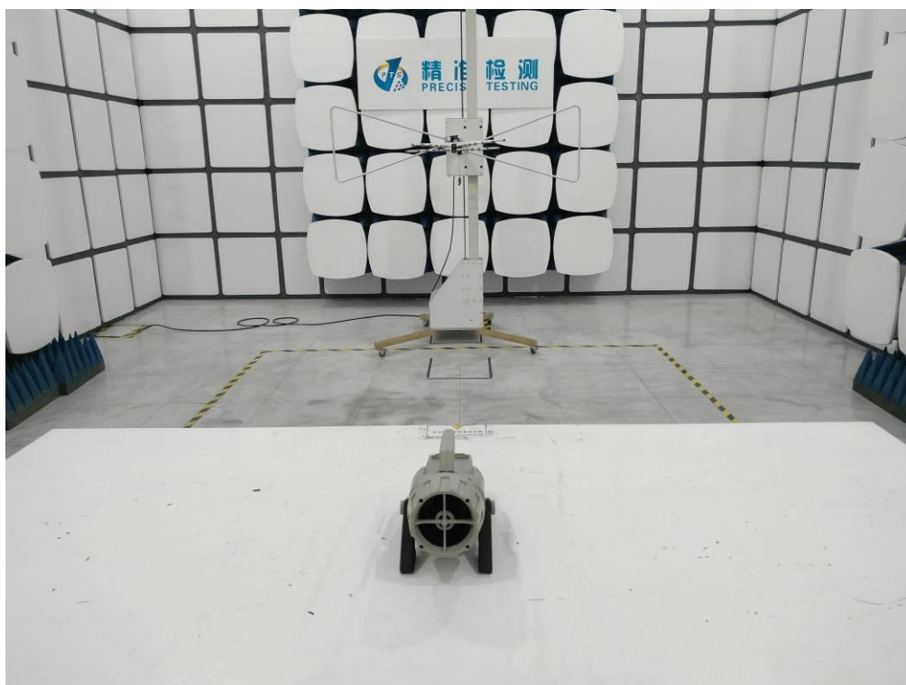
RADIATED EMISSION TEST SETUP BELOW 1GHz-Mode 2
