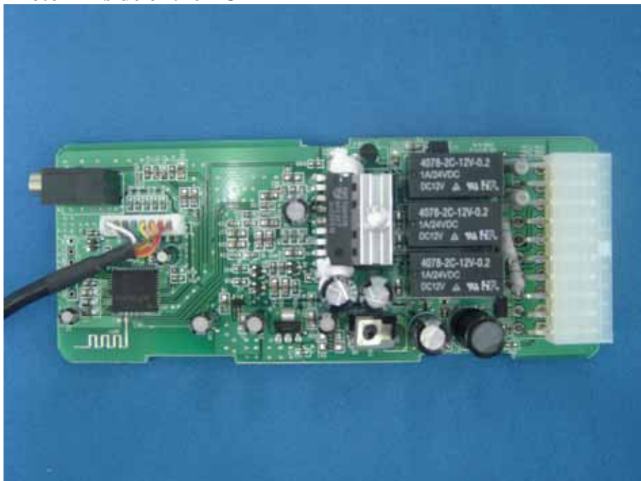
Photo 4 Inside of the EUT
