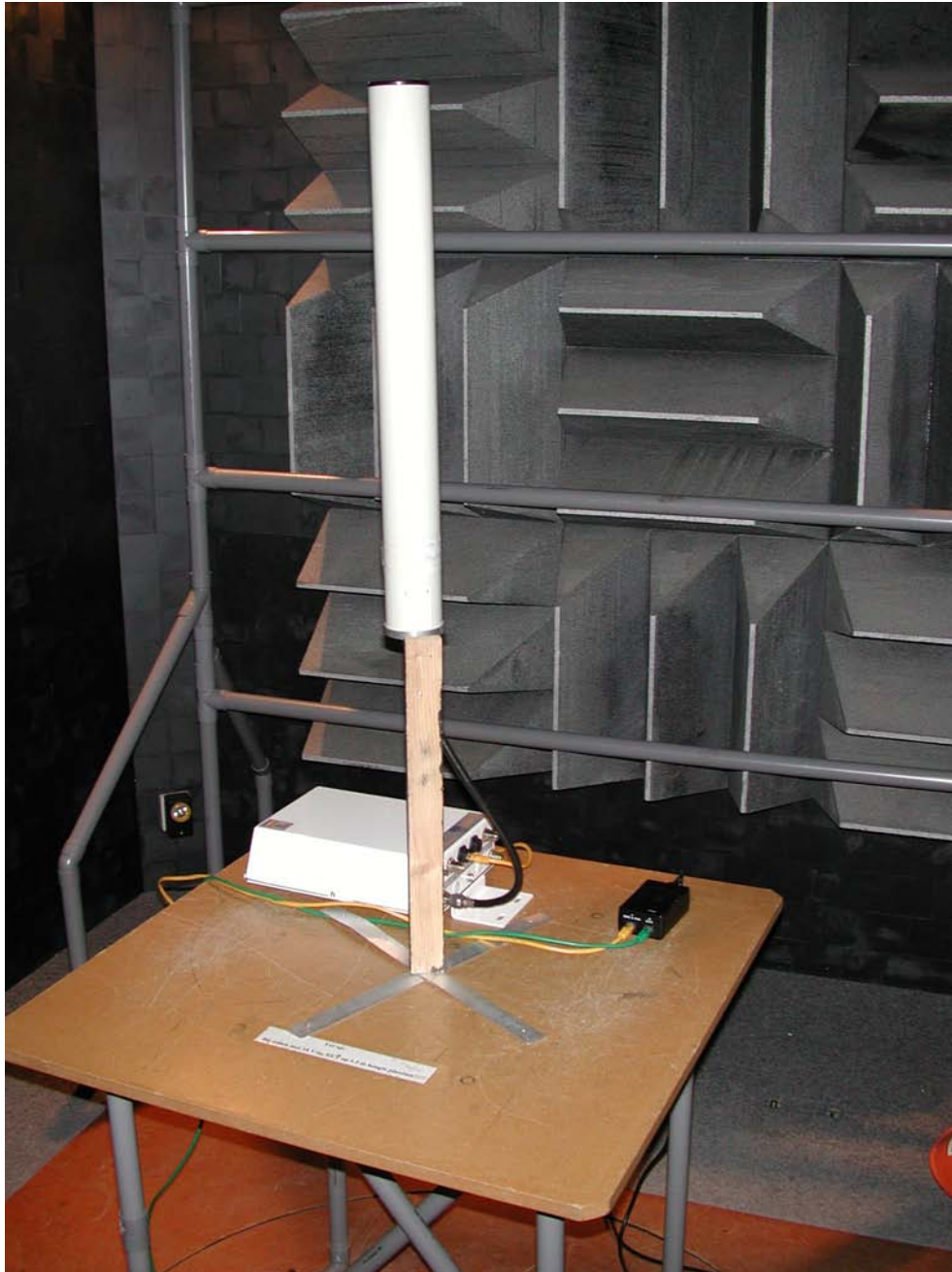
Photograph 1: Test setup radiated measurements 802.11 b/g
