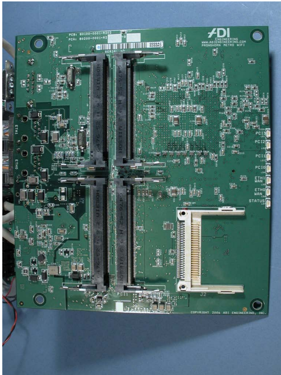
Photograph 2: Mainboard, Pronghorn Metro Top (stripped)
