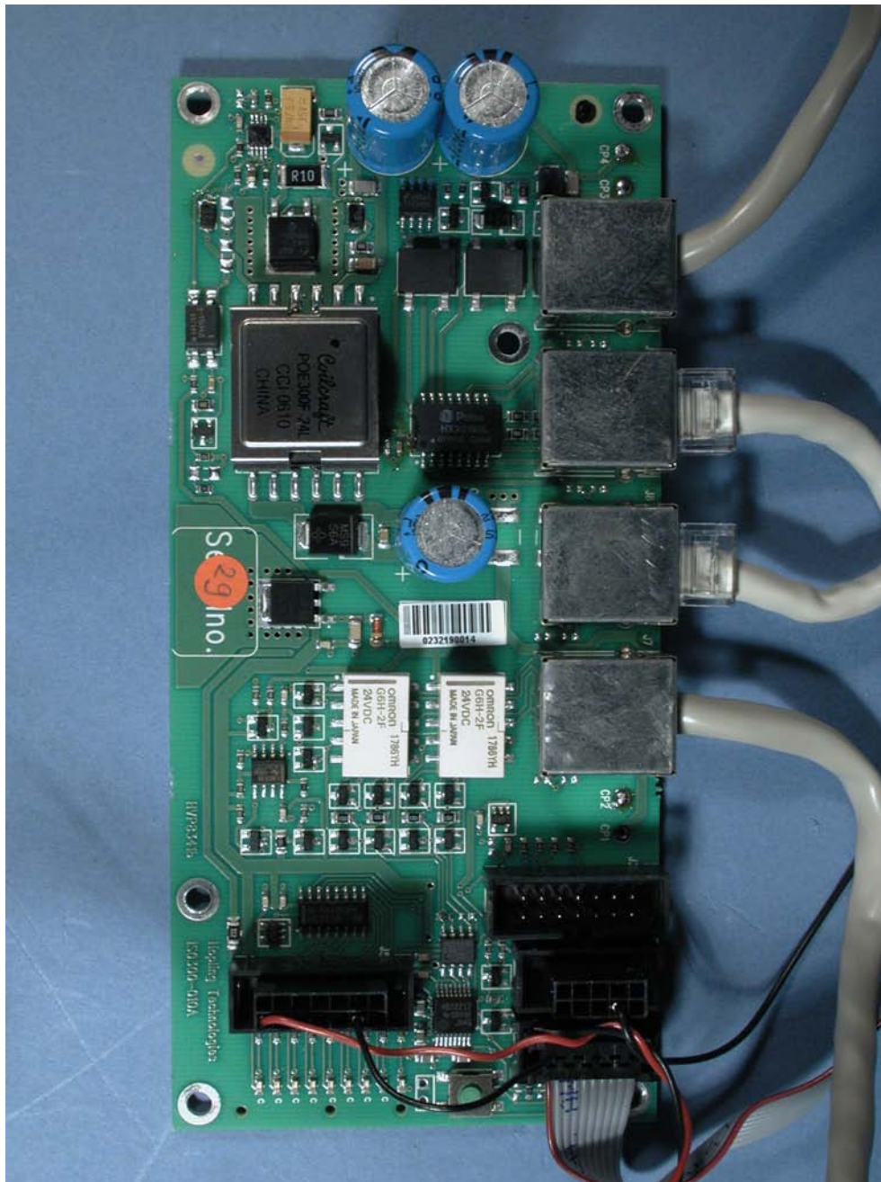
Photograph 8: DTS module top view
