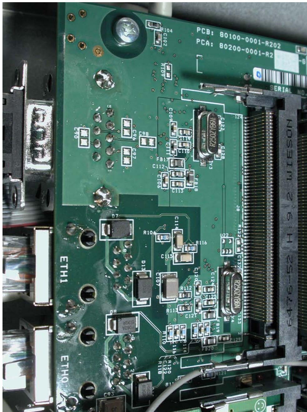
Photograph 3: Mainboard, Pronghorn Metro radio module-slot
