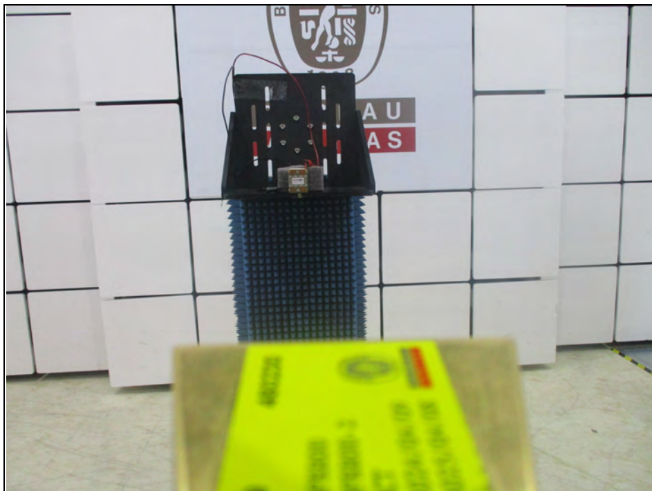
Radiated Emission Test (50GHz ~ 55GHz)
