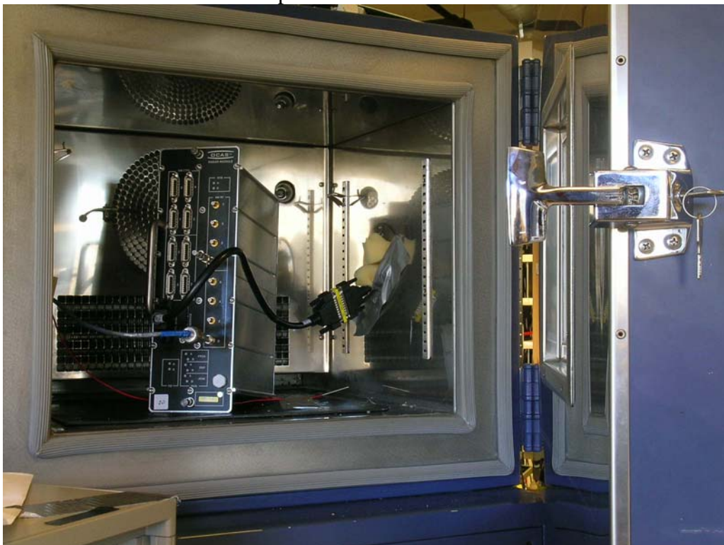
Test set-up for climatic measurements
