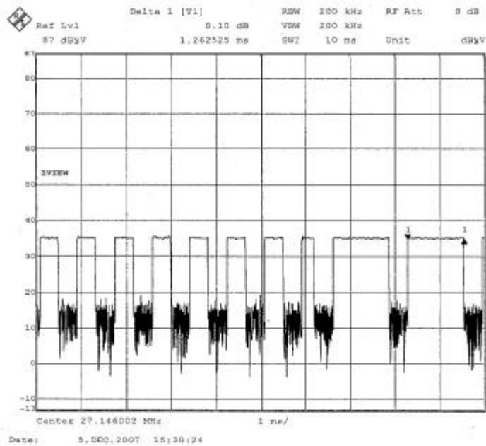
Figure B [Long Pulse]
