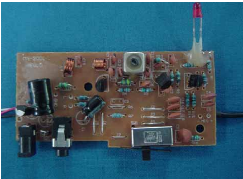
Photo4 Inside of the EUT
