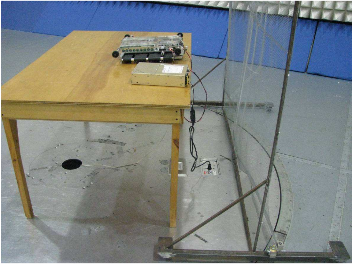
Conducted Emissions
