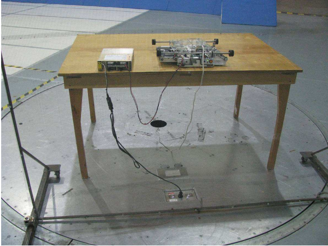
Conducted Emissions
