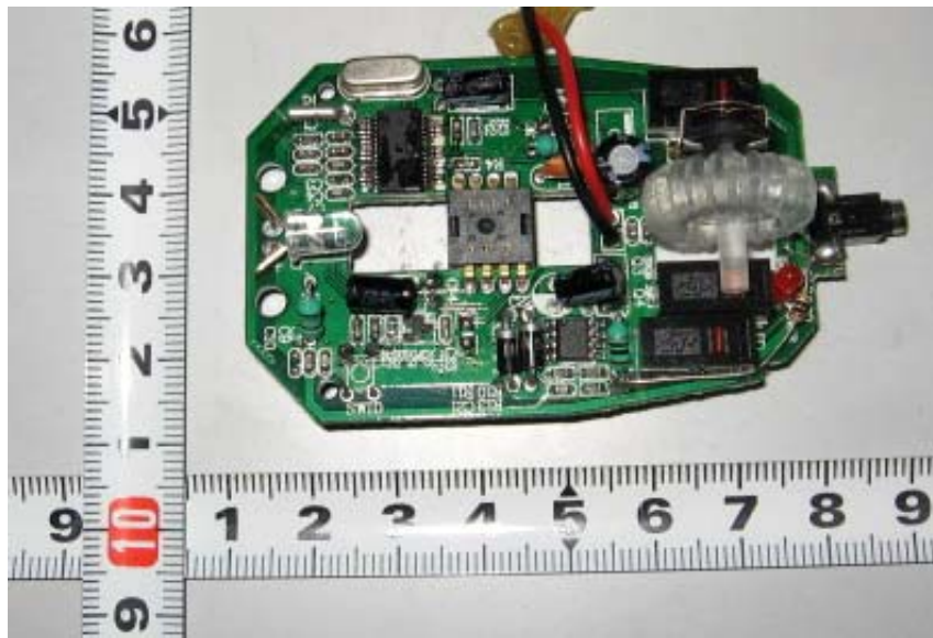
EUT – PCB View (Transmitter)
