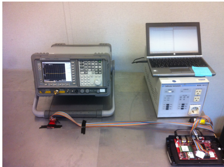
FIGURE 4 - CONDUCTED RF
