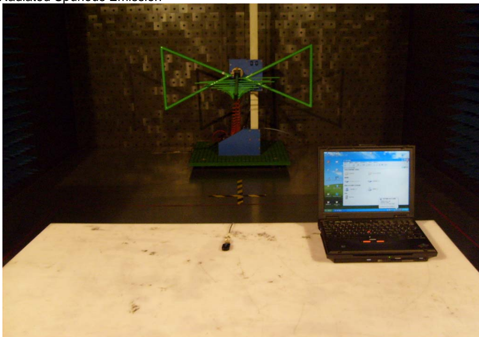
Radiated Spurious Emission
