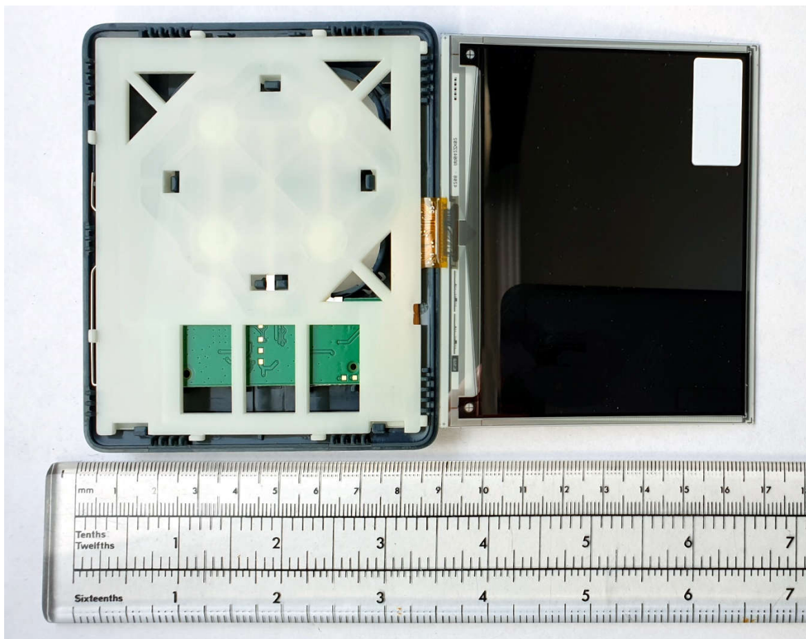
DD42-3A (Chroma Aeon 42) – Front View, with Front Cover removed and display “flipped” to reveal PCB.
