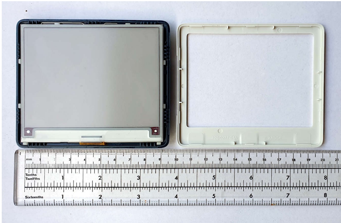
DD42-3A (Chroma Aeon 42) – Front View, with Front Cover removed.
