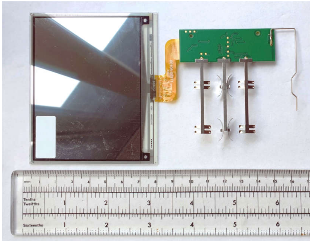
DD42-3A (Chroma Aeon 42) – PCB and Display Glass Rear View.
