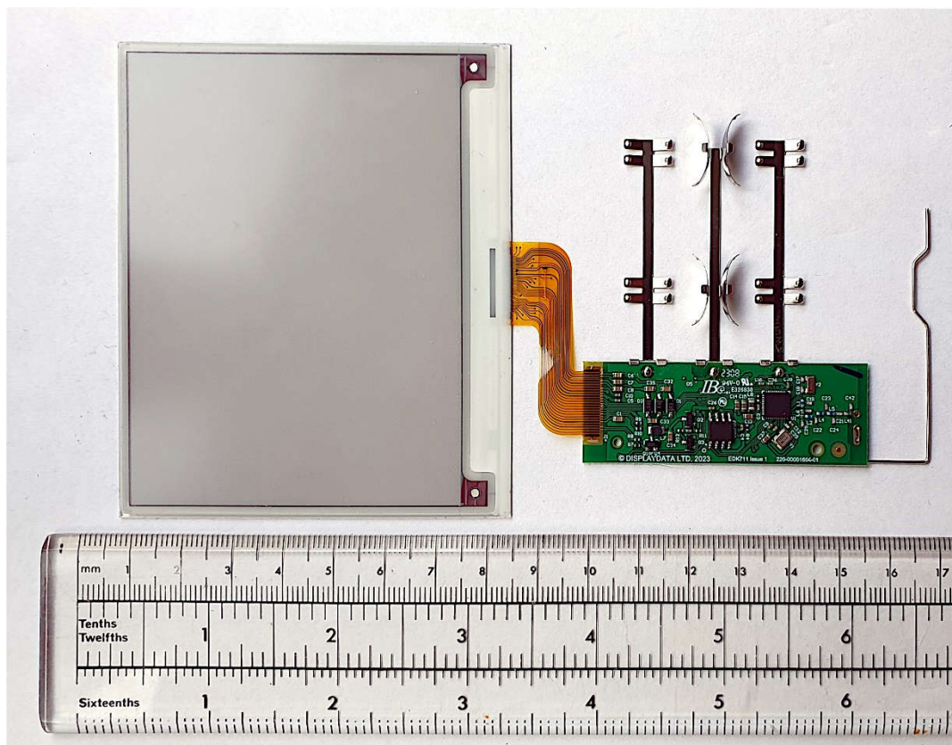
DD42-3A (Chroma Aeon 42) – PCB and Display Glass Front View.
