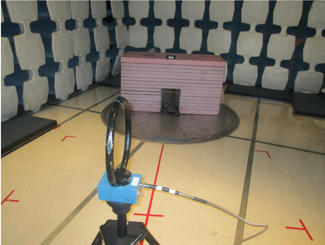
Radiated Emissions 9kHz - 30MHz
