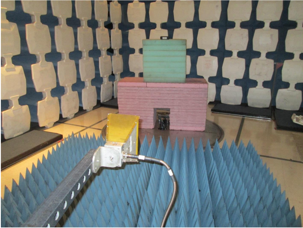
Radiated Emissions 1GHz – 6GHz
