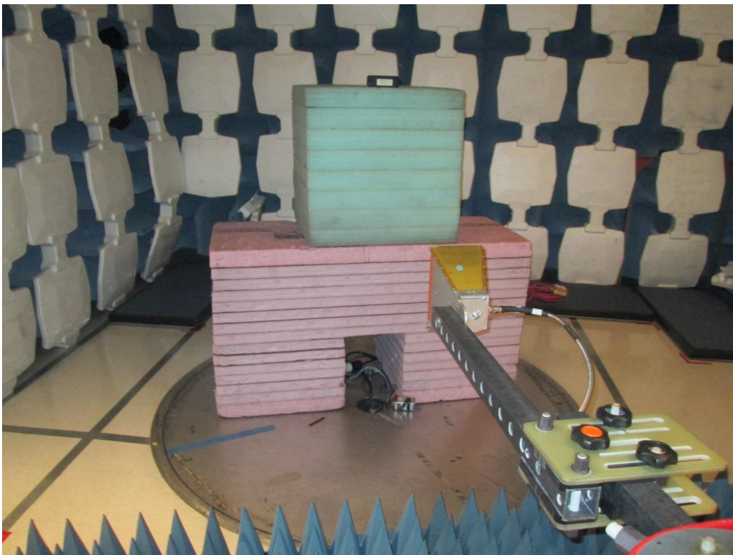
Radiated Emissions 6GHz – 18GHz
