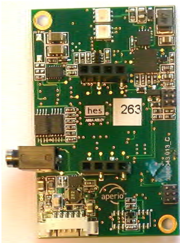
K100-622-PA2 main board – top view
