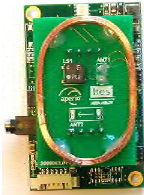
K100-622-PA2 antenna board mounted on main board - front view
