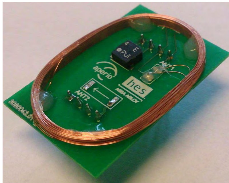
KS100-640-PA2 antenna board – side view
