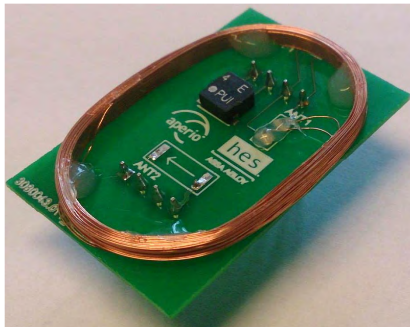
K100-622-PA2 antenna board – side view
