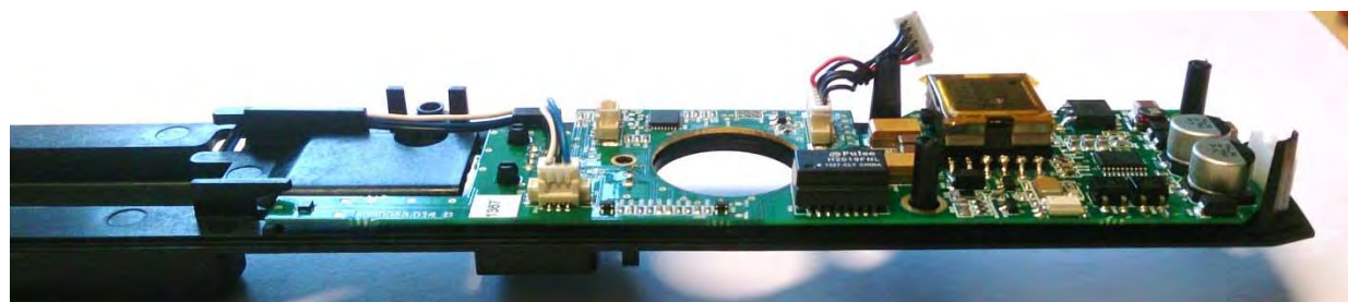
KS100-640-PA2 secure board on rear plate – side view
