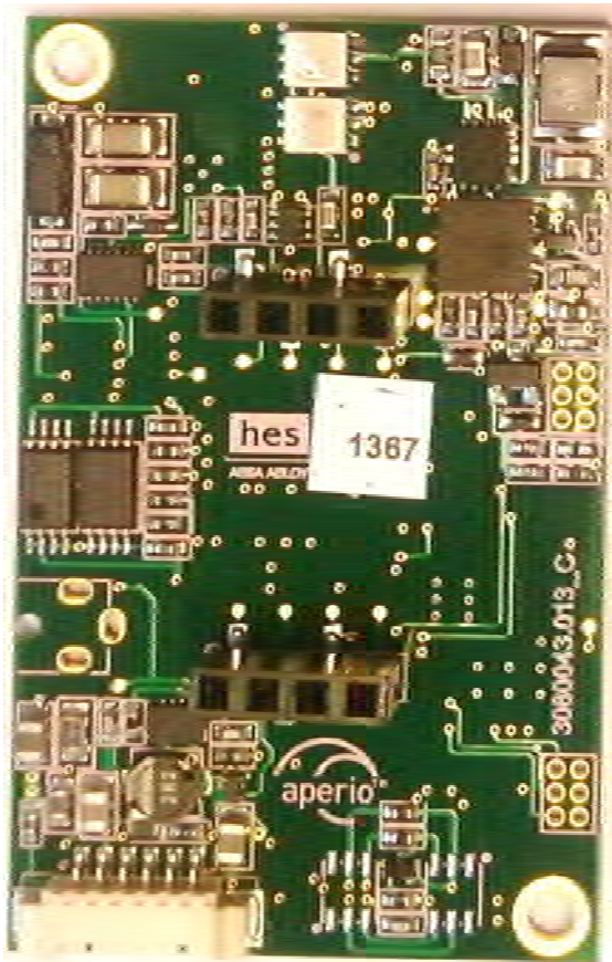
KS100-640-PA2 main board – top view
