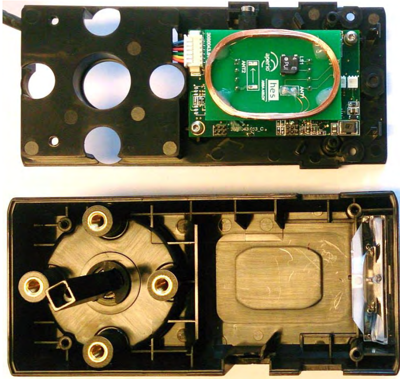
K100-622-PA2 Reader front view
