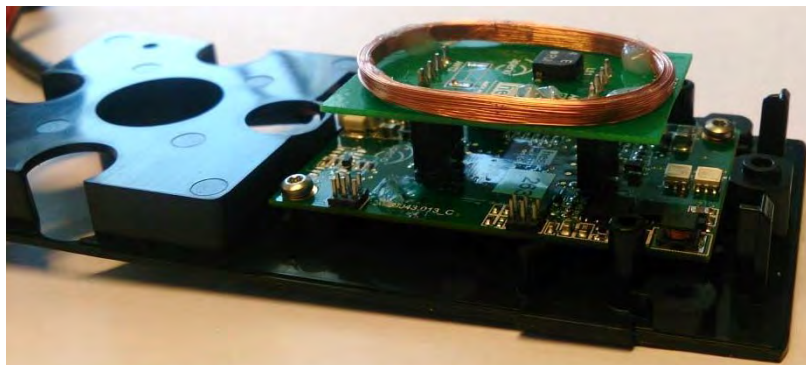
K100-622-PA2 Reader side view
