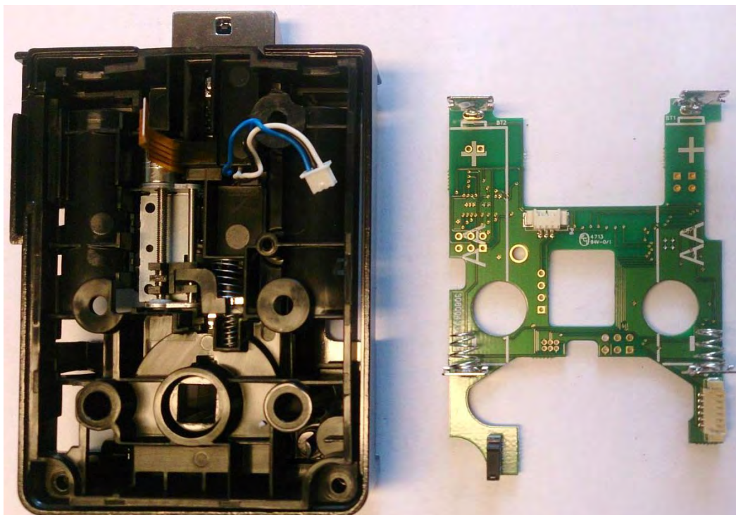
K100-622-PA2 Lock body secure board removed
