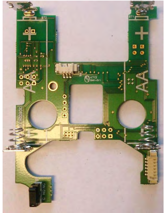
K100-622-PA2 Lock body secure board rear view
