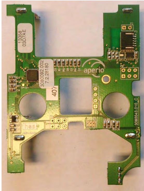
K100-622-PA2 Lock body secure board top view
