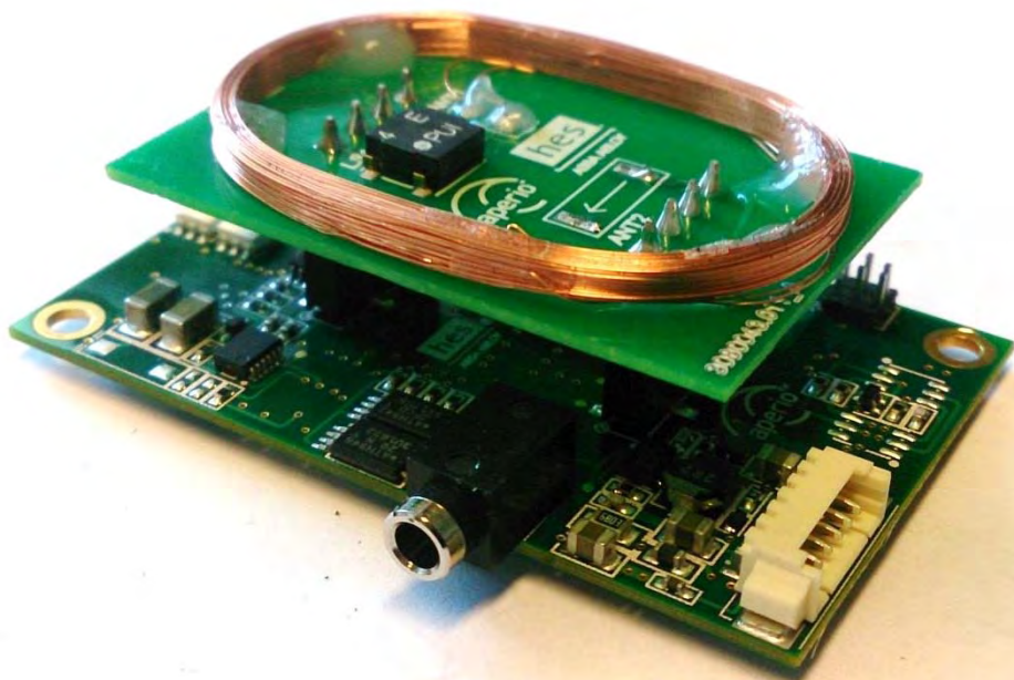
K100-622-PA2 antenna board mounted on main board – side view
