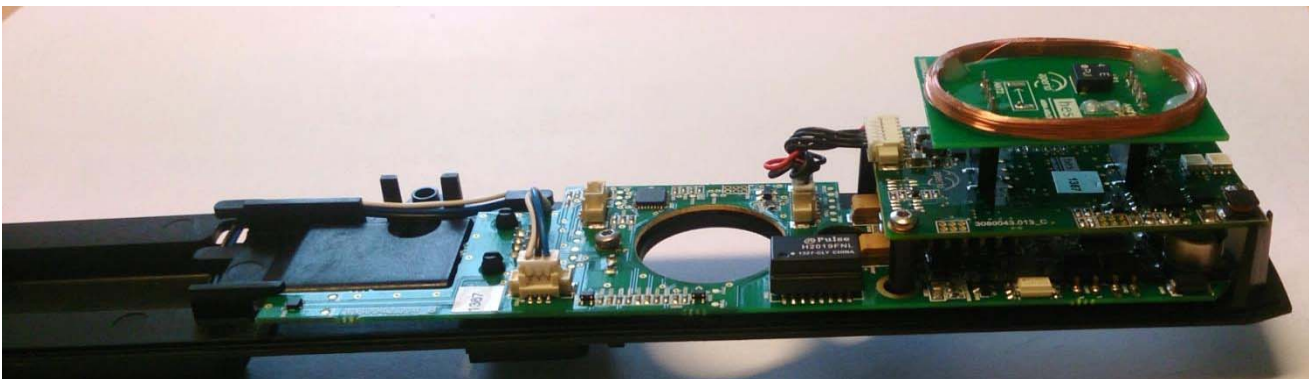
KS100-640-PA2 side view
