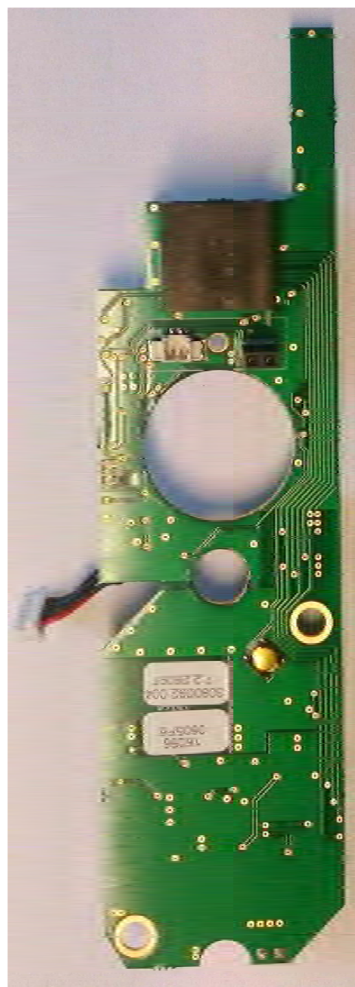
KS100-640-PA2 secure board – rear view
