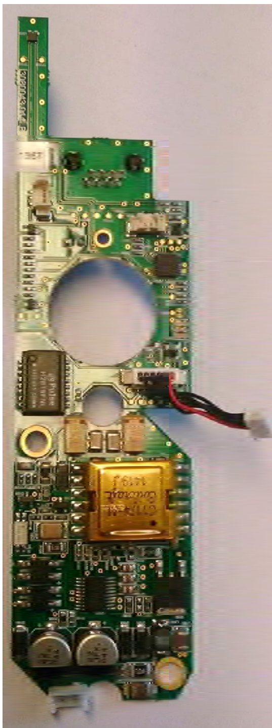
KS100-640-PA2 secure board – top view
