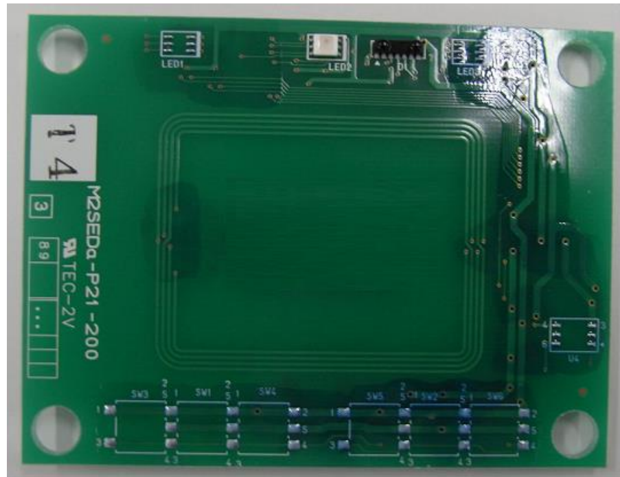
TOP View
