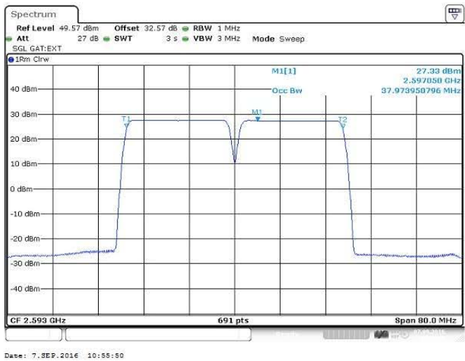
Figure 47 Occupied Bandwidth–QPSK (2583/ 2603 MHz) (2 X 20 MHz Channel BW)
