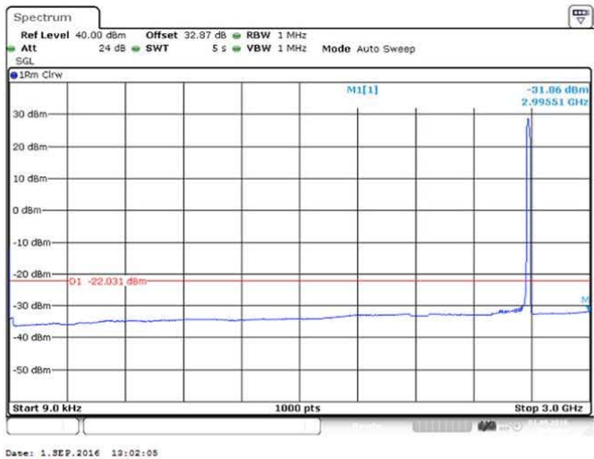
Figure 93 Spurious Emissions (9kHz – 3GHz) – 16QAM (2593.0 MHz) (20MHz Channel BW)
