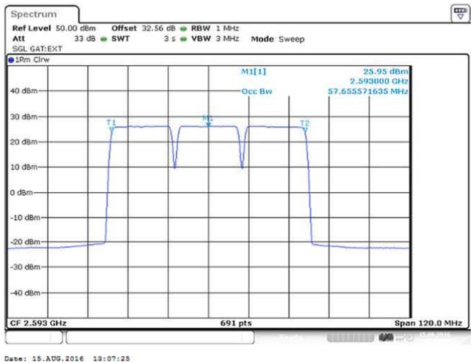
Figure 60 Occupied Bandwidth–64QAM (2573/ 2593/ 2613 MHz) (3 X 20 MHz Channel BW)
