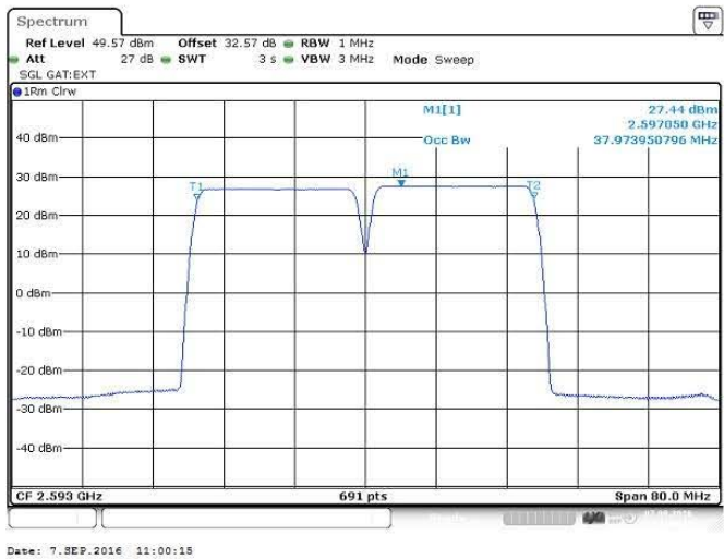
Figure 48 Occupied Bandwidth–64QAM (2583/ 2603 MHz) (2 X 20 MHz Channel BW)
