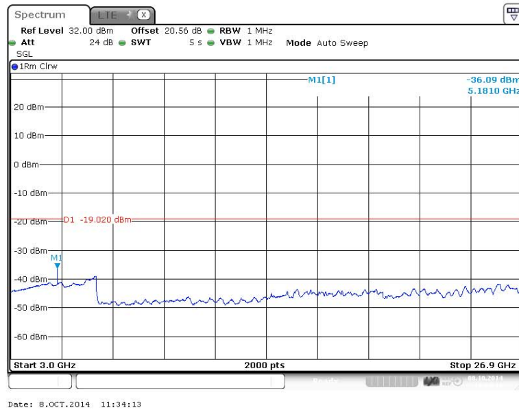
Figure 66 Spurious Emissions (3GHz – 26.900GHz) – 16QAM (2593.0 MHz) (10MHz Channel BW)
