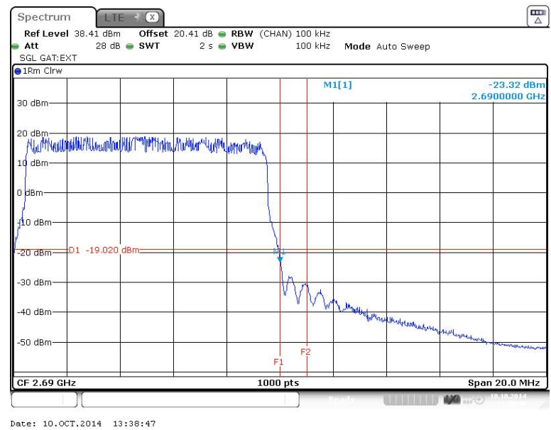
Figure 64 Spurious Emissions (Upper Band Edge) – 16QAM (2685.0 MHz) (10MHz Channel BW)
