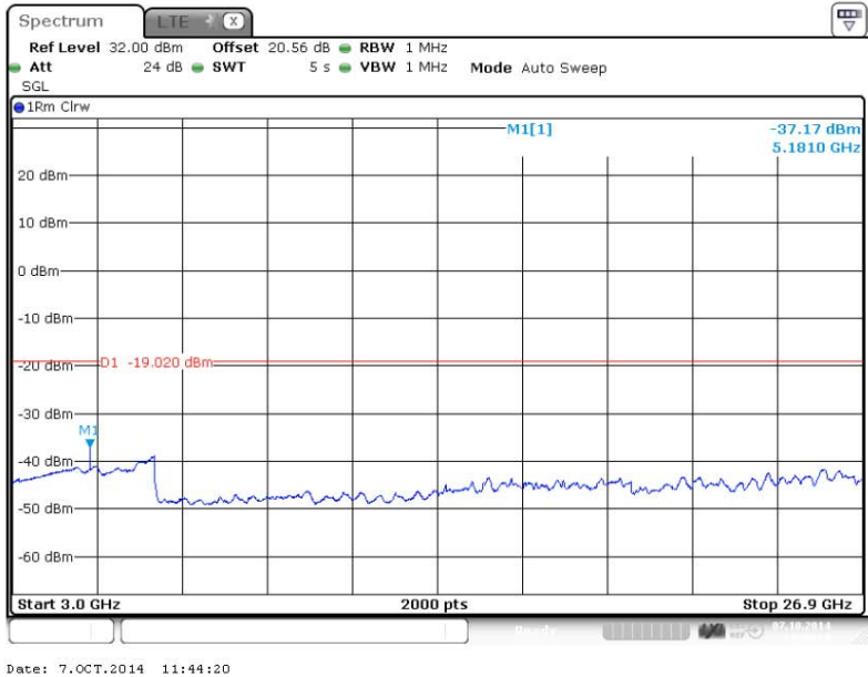
Figure 86 Spurious Emissions (3GHz – 26.900GHz) – QPSK (2593.0 MHz) (10MHz Channel BW)
