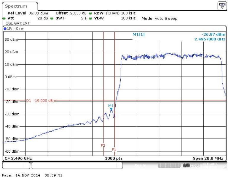
Figure 87 Spurious Emissions (Lower Band Edge) – 16QAM (2501.1 MHz) (10MHz Channel BW)
