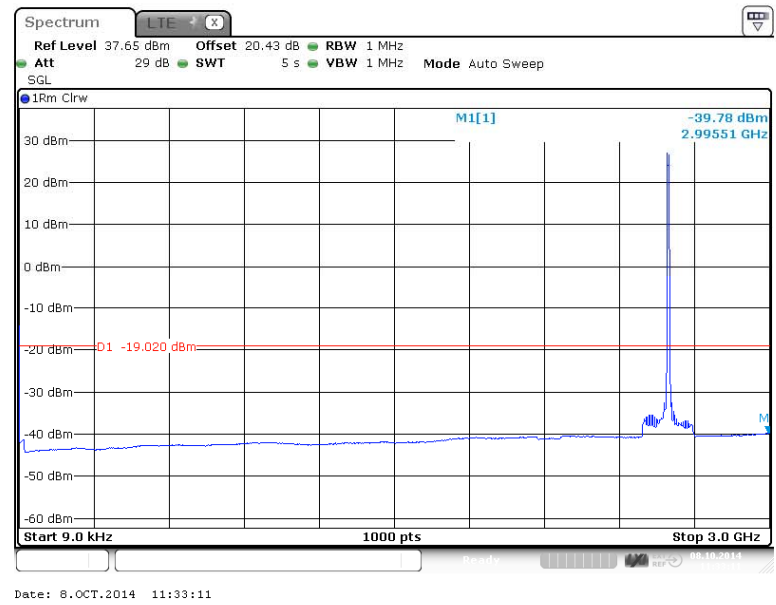
Figure 65 Spurious Emissions (9kHz – 3GHz) – 16QAM (2593.0 MHz) (10MHz Channel BW)
