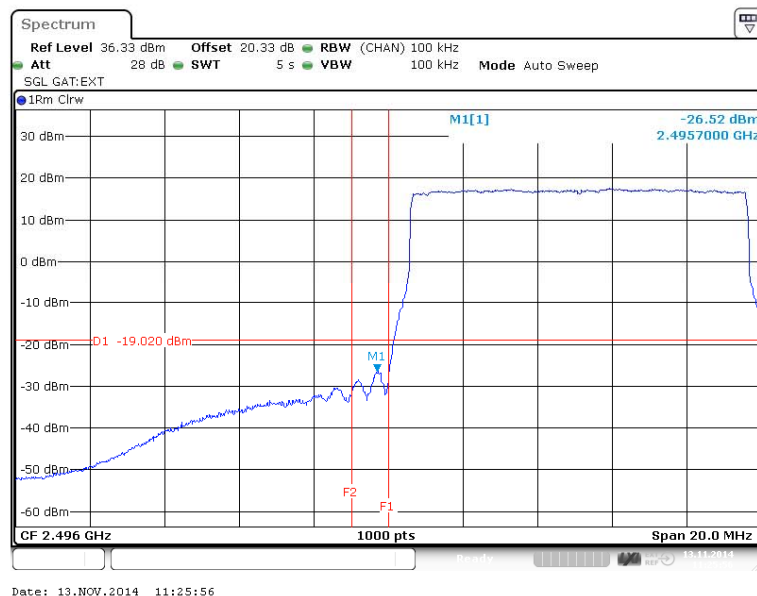
Figure 67 Spurious Emissions (Lower Band Edge) – 64QAM (2501.1 MHz) (10MHz Channel BW)
