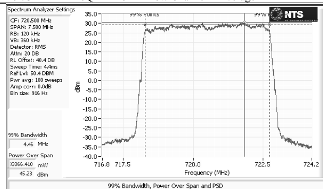
Port 3 – LTE – 64QAM – 5M – Low Channel – Average
