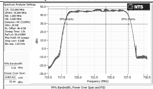
Port 3 – LTE – 16QAM – 10M – Center Channel – Peak
