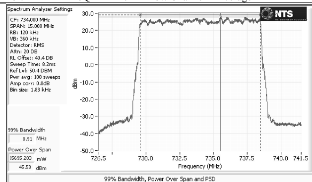
Port 2 – LTE – 64QAM – 10M – Low Channel – Average
