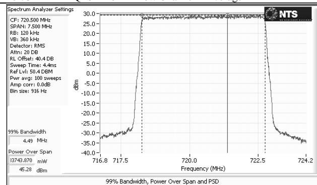
Port 3 – LTE – 16QAM – 5M – Low Channel – Average
