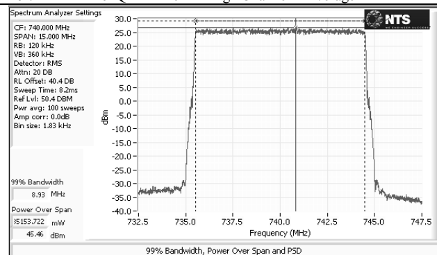
Port 2 - LTE - 64QAM - 10M - High Channel - Average
