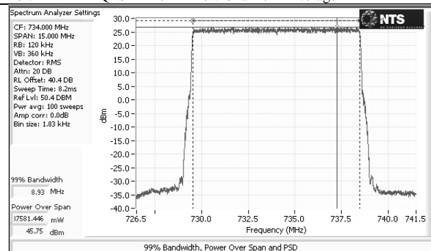
Port 2 – LTE – 16QAM – 10M – Low Channel – Average
