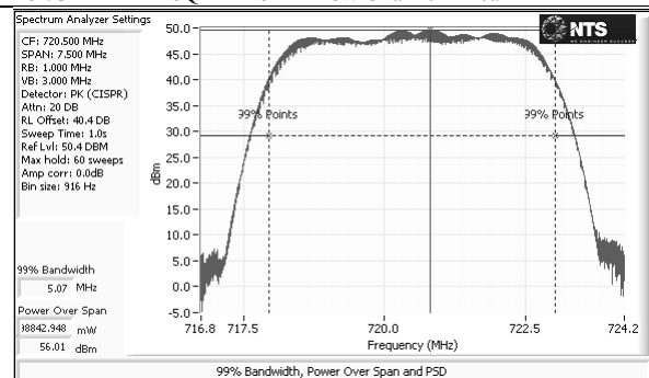
Port 3 – LTE – 16QAM – 5M – Low Channel – Peak
