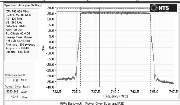
Port 2 - LTE - 16QAM - 10M - High Channel - Average
