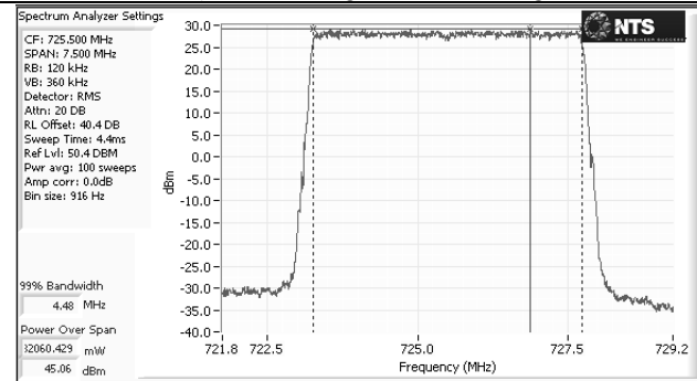
Port 3 - LTE - 64QAM - 5M - High Channel - Average
