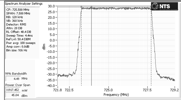
Port 3 - LTE - 16QAM - 5M - High Channel - Average
