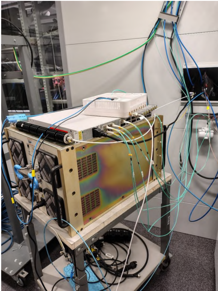
Figure 1 - Conducted test setup
