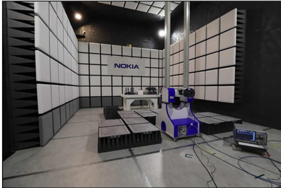
Figure 7 - Radiated Emissions (18 GHz to 40 GHz)
