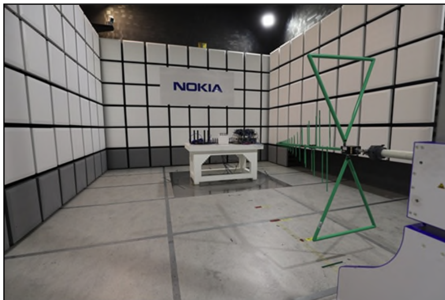
Figure 3 - Radiated Emissions (30 MHz to 1 GHz)
