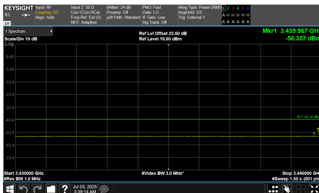
Test Case C 3430.0 MHz to 3440.0 MHz
