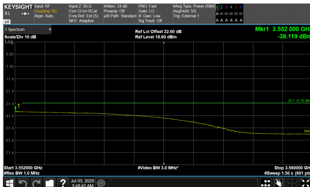
Test Case C 3552.0 MHz to 3560.0 MHz
