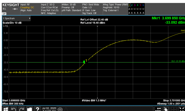
QPSK Modulation 30 MHz Channel Bandwidth Low Channel, 3715.02 MHz 3699.0 MHz to 3701.0 MHz
