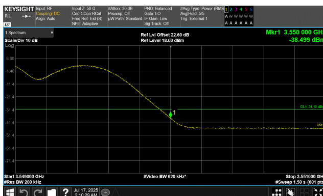
QPSK Modulation 50 MHz Channel Bandwidth High Channel, 3525.00 MHz 3549.0 MHz to 3551.0 MHz
