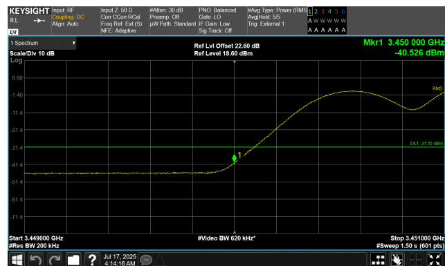
Test Case A 3449.0 MHz to 3451.0 MHz
