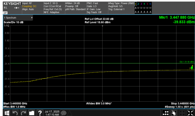
QPSK Modulation 50 MHz Channel Bandwidth Low Channel, 3475.02 MHz 3440.0 MHz to 3448.0 MHz
