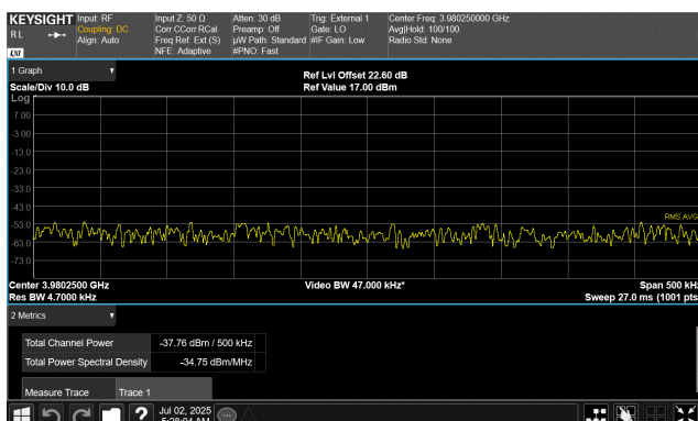
QPSK Modulation 50 MHz Channel Bandwidth High Channel, 3954.99 MHz 3980.0 MHz to 3980.5 MHz
