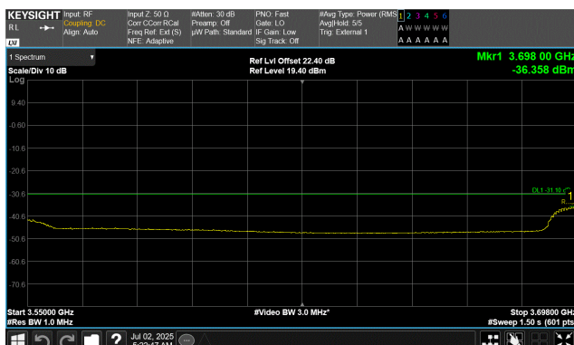
QPSK Modulation 50 MHz Channel Bandwidth Low Channel, 3725.01 MHz 3550.0 MHz to 3698.0 MHz
