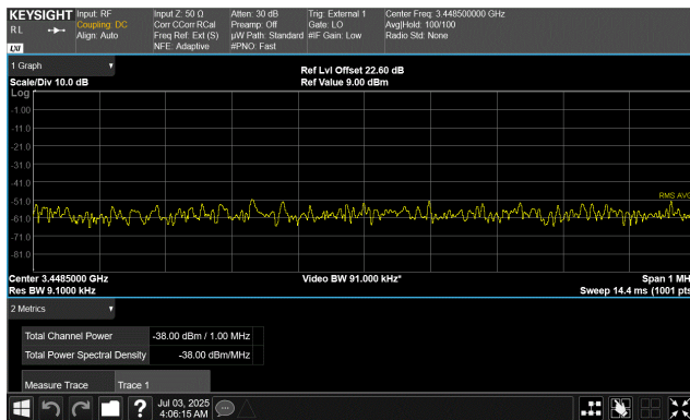
Test Case D 3448.0 MHz to 3449.0 MHz
