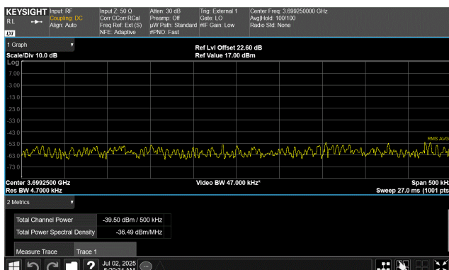
QPSK Modulation 50 MHz Channel Bandwidth Low Channel, 3725.01 MHz 3699.0 MHz to 3699.5 MHz
