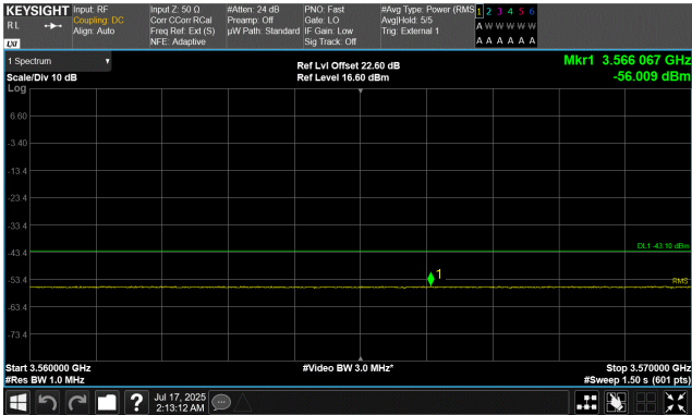
QPSK Modulation 50 MHz Channel Bandwidth High Channel, 3525.00 MHz 3560.0 MHz to 3570.0 MHz
