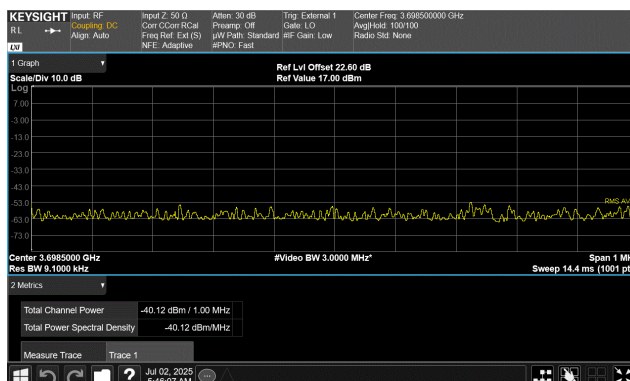
QPSK Modulation 30 MHz Channel Bandwidth Low Channel, 3715.02 MHz 3698.0 MHz to 3699.0 MHz
