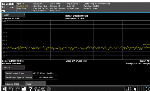
QPSK Modulation 50 MHz Channel Bandwidth Low Channel, 3475.02 MHz 3448.0 MHz to 3449.0 MHz
