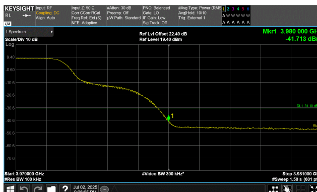
QPSK Modulation 10 MHz Channel Bandwidth High Channel, 3975.00 MHz 3979.0 MHz to 3981.0 MHz
