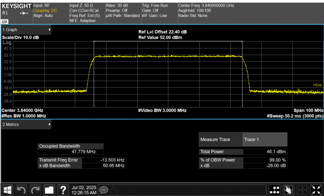
Port 1 50 MHz Channel Bandwidth 256QAM Modulation Middle Channel, 3840.00 MHz
