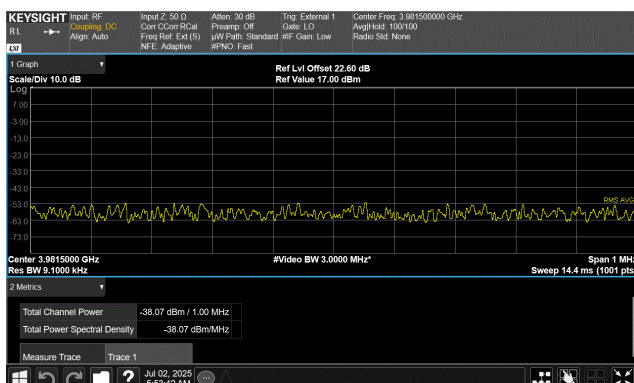
QPSK Modulation 30 MHz Channel Bandwidth High Channel, 3964.98 MHz 3981.0 MHz to 3982.0 MHz
