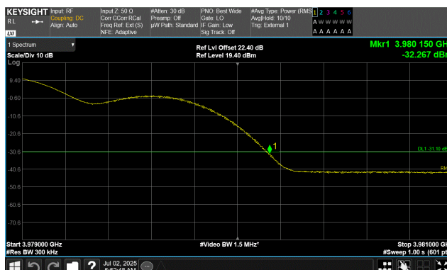
QPSK Modulation 30 MHz Channel Bandwidth High Channel, 3964.98 MHz 3979.0 MHz to 3981.0 MHz
