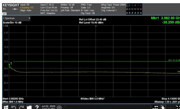
QPSK Modulation 10 MHz Channel Bandwidth High Channel, 3975.00 MHz 3982.0 MHz to 4130.0 MHz
