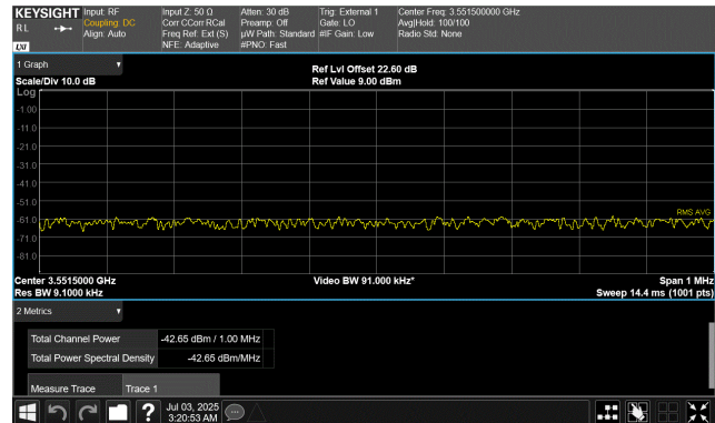
Test Case B 3551.0 MHz to 3552.0 MHz
