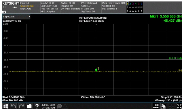
Test Case B 3549.0 MHz to 3551.0 MHz
