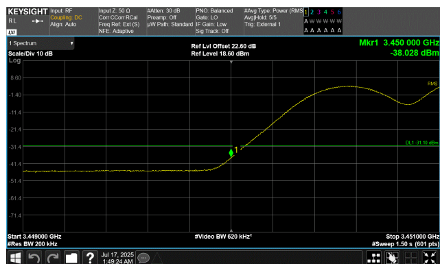
QPSK Modulation 50 MHz Channel Bandwidth Low Channel, 3475.02 MHz 3449.0 MHz to 3451.0 MHz
