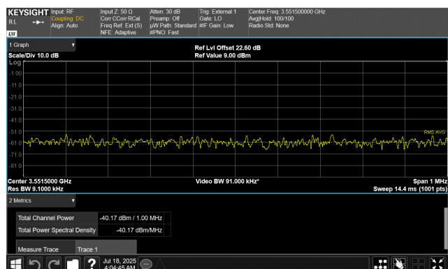
QPSK Modulation 50 MHz Channel Bandwidth High Channel, 3525.00 MHz 3551.0 MHz to 3552.0 MHz
