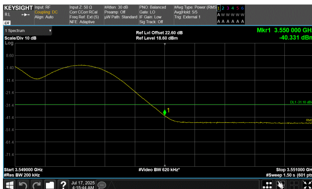
Test Case A 3549.0 MHz to 3551.0 MHz
