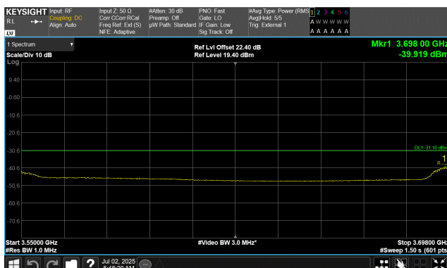
QPSK Modulation 30 MHz Channel Bandwidth Low Channel, 3715.02 MHz 3550.0 MHz to 3698.0 MHz
