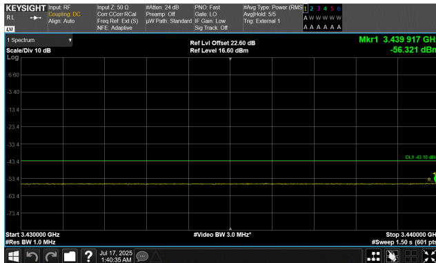
QPSK Modulation 50 MHz Channel Bandwidth Low Channel, 3475.02 MHz 3430.0 MHz to 3440.0 MHz
