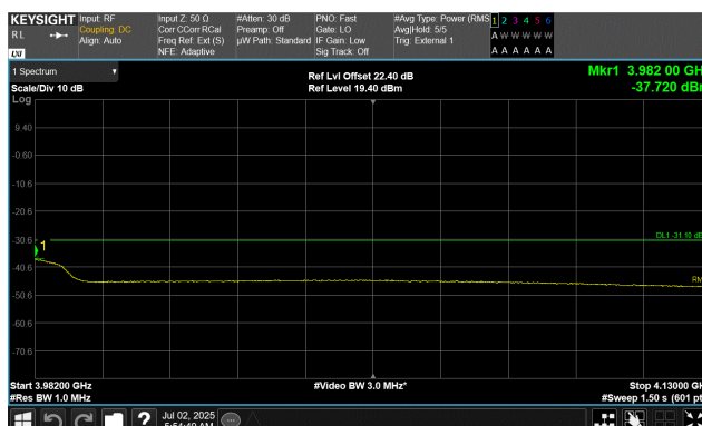
QPSK Modulation 30 MHz Channel Bandwidth High Channel, 3964.98 MHz 3982.0 MHz to 4130.0 MHz
