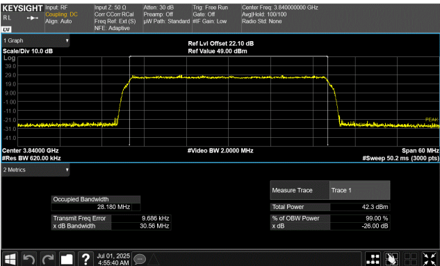
Port 1 30 MHz Channel Bandwidth 256QAM Modulation Middle Channel, 3840.00 MHz
