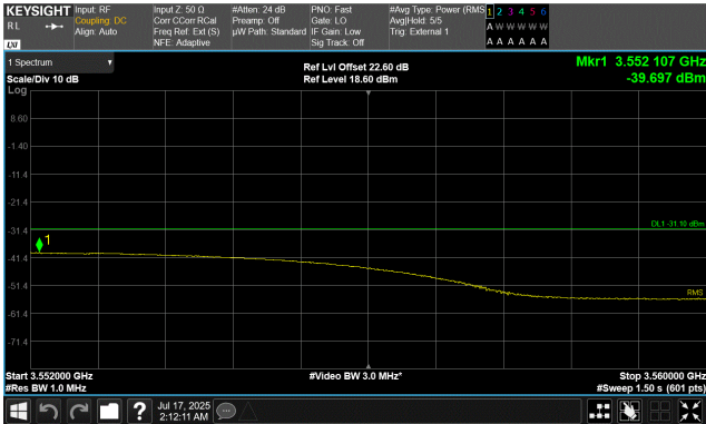
QPSK Modulation 50 MHz Channel Bandwidth High Channel, 3525.00 MHz 3552.0 MHz to 3560.0 MHz
