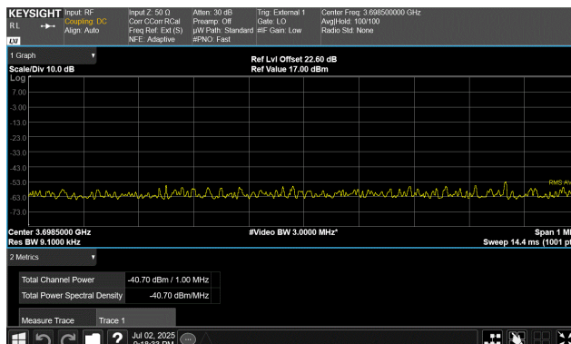
QPSK Modulation 10 MHz Channel Bandwidth Low Channel, 3705.00 MHz 3698.0 MHz to 3699.0 MHz
