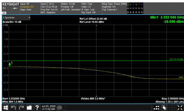
Test Case D 3552.0 MHz to 3560.0 MHz
