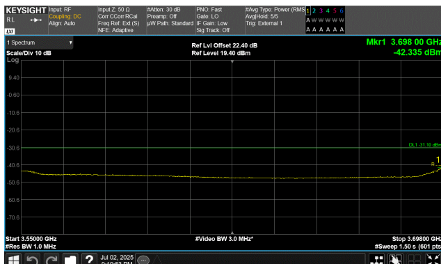
QPSK Modulation 10 MHz Channel Bandwidth Low Channel, 3705.00 MHz 3550.0 MHz to 3698.0 MHz
