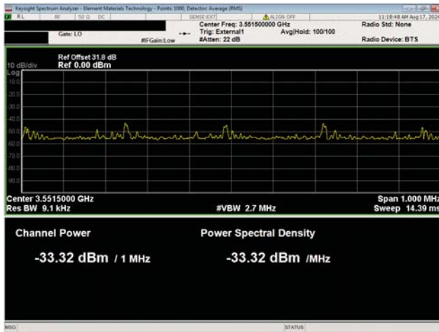
Port 1 QPSK Modulation Test Case 2
