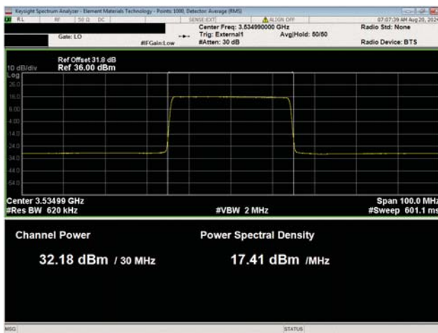
Port 1 30 MHz Channel Bandwidth QPSK Modulation High Channel, 3534.99 MHz
