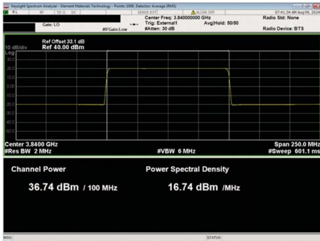
100 MHz Channel Bandwidth QPSK Modulation Middle Channel, 3840.00 MHz Port 5
