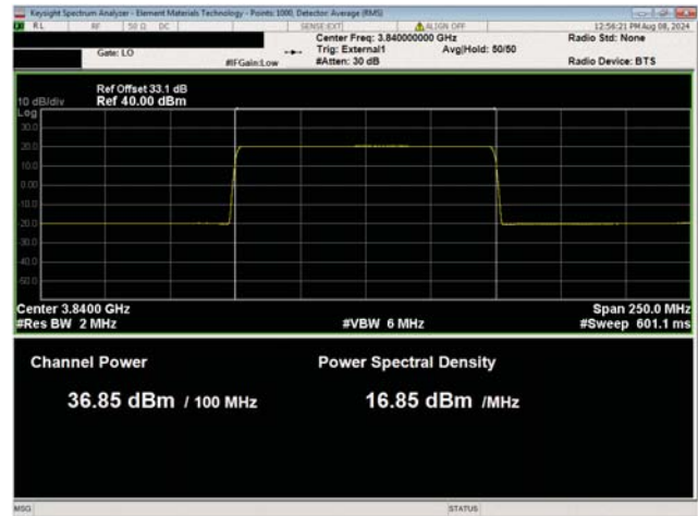
100 MHz Channel Bandwidth QPSK Modulation Middle Channel, 3840.00 MHz Port 58
