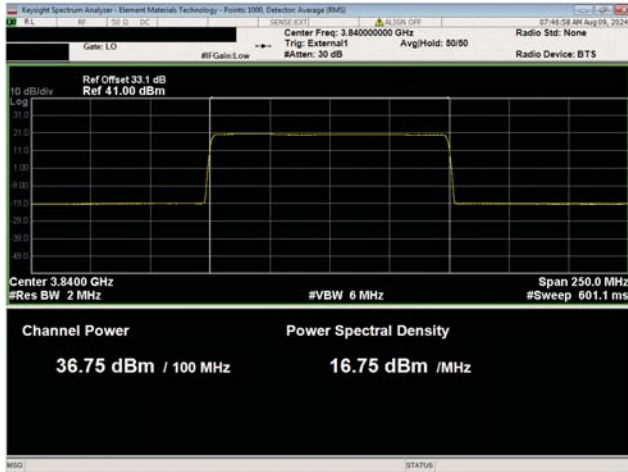
100 MHz Channel Bandwidth QPSK Modulation Middle Channel, 3840.00 MHz Port 37
