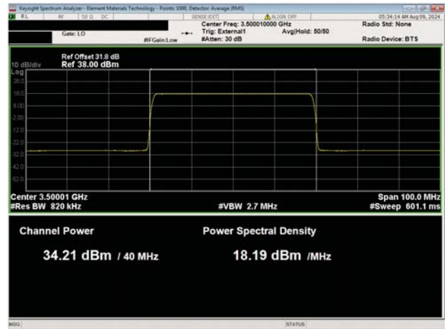
40 MHz Channel Bandwidth QPSK Modulation Middle Channel, 3500.01 MHz Port 30
