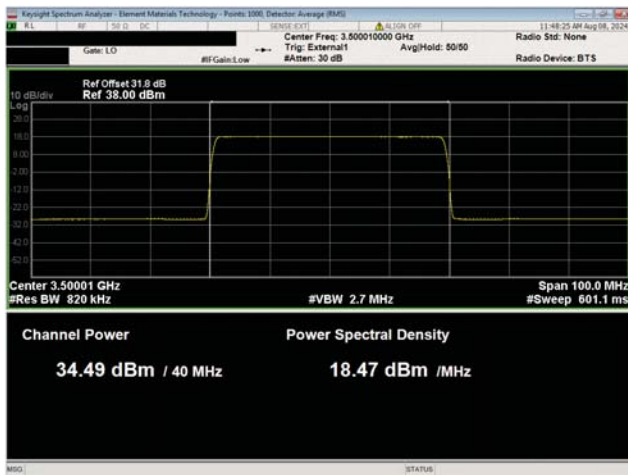
40 MHz Channel Bandwidth QPSK Modulation Middle Channel, 3500.01 MHz Port 55
