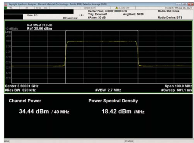
40 MHz Channel Bandwidth QPSK Modulation Middle Channel, 3500.01 MHz Port 28
