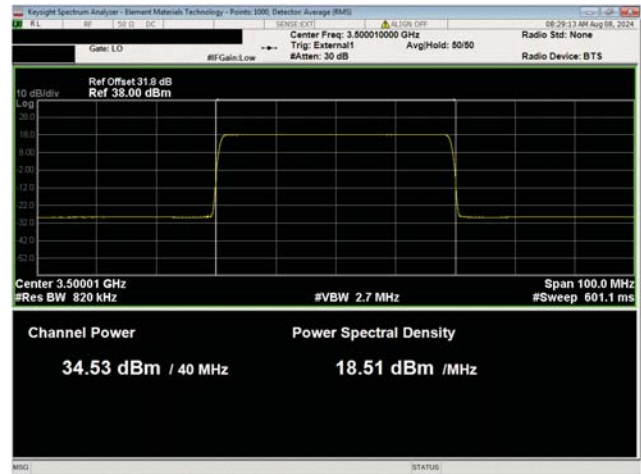
40 MHz Channel Bandwidth QPSK Modulation Middle Channel, 3500.01 MHz Port 50
