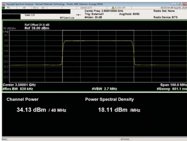
40 MHz Channel Bandwidth QPSK Modulation Middle Channel, 3500.01 MHz Port 31
