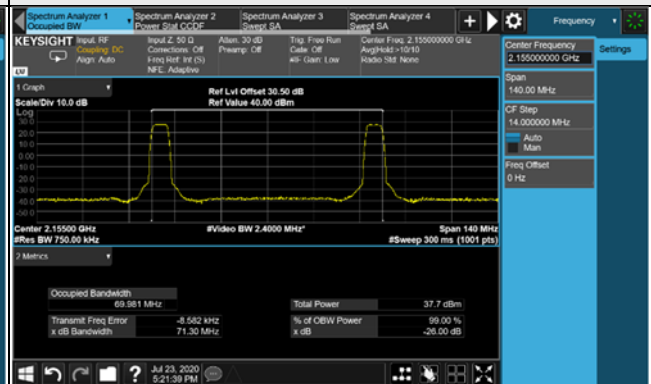
Chain 3 / 16QAM
