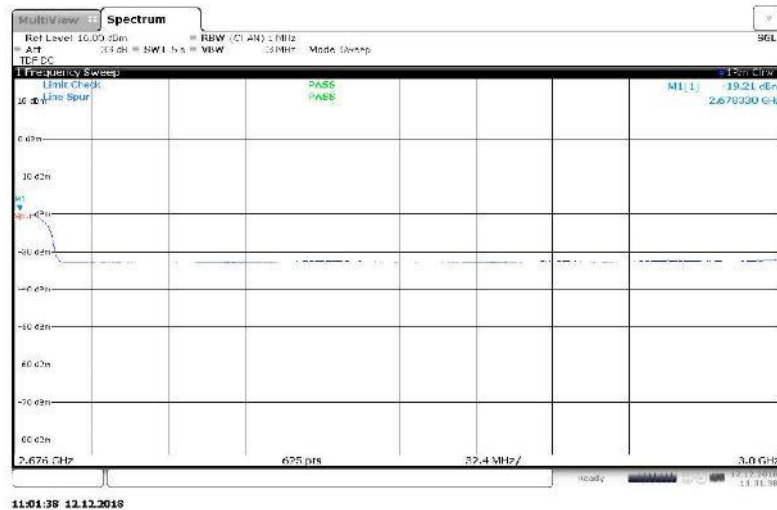
Figure 186 Spurious Emissions (2.676 GHz – 3 GHz) – 64QAM (2645 MHz, 2665 MHz, 2x20 MHz Channel BW)
