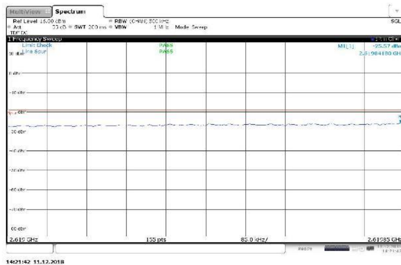
Figure 147 Spurious Emissions (Lower Band Edge) – QPSK (2627.5 MHz, 2642.5 MHz, 2x15 MHz Channel BW)
