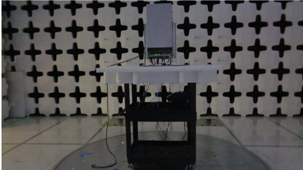
Radiated Spurious
