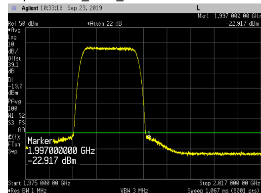
Top Channel_ UBE_ 1975 to 2017MHz
