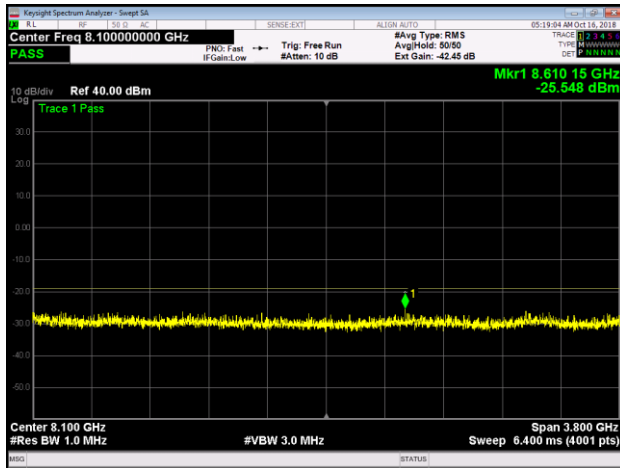
Band 25, LTE10, T, Lower, 6200MHz-10GHz
