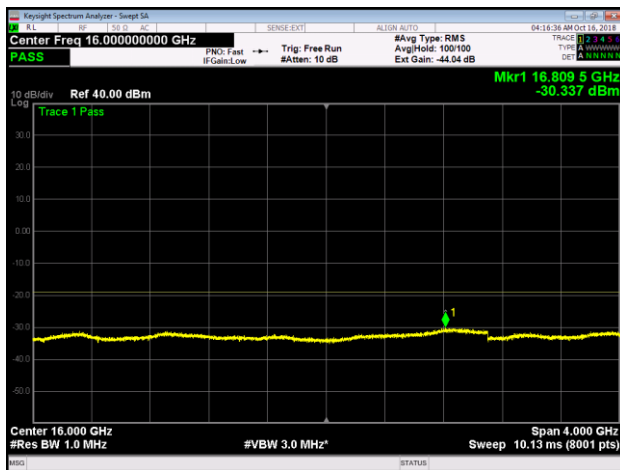
Band 25, LTE10, B, Lower, 14GHz-18GHz
