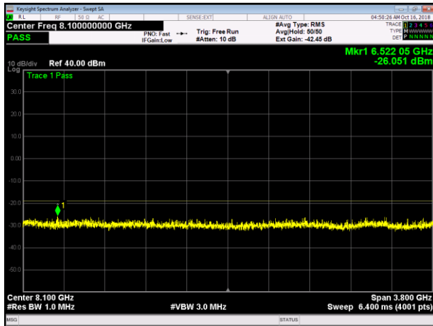
Band 25, LTE10, M, Upper, 6200MHz-10GHz
