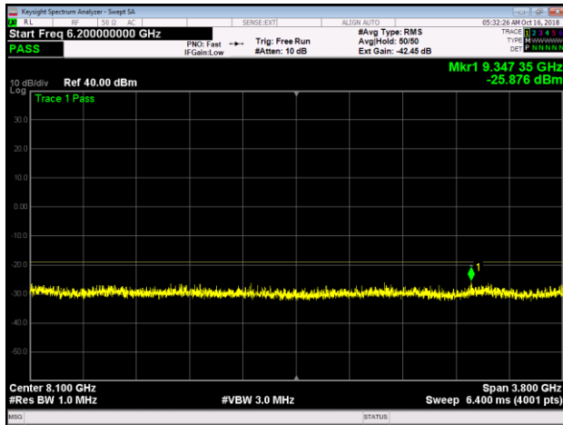
Band 66, LTE10, B, Lower, 6200MHz-10GHz
