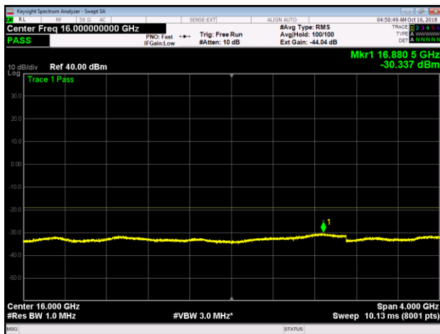
Band 25, LTE10, M, Upper, 14GHz-18GHz
