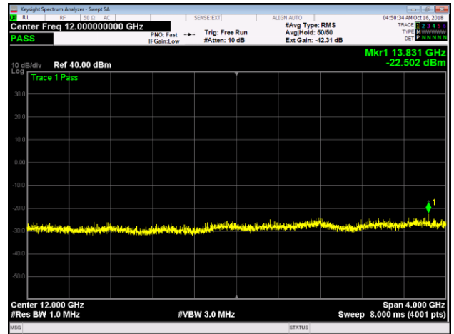
Band 25, LTE10, M, Upper, 10GHz-14GHz
