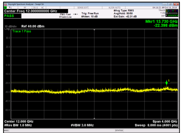
Band 25, LTE10, B, Lower, 10GHz-14GHz
