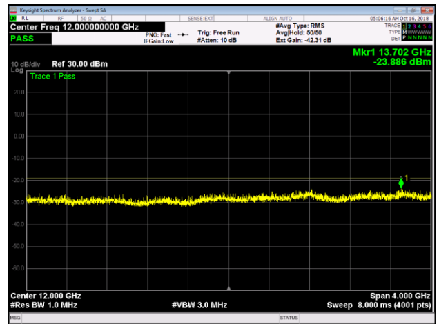
Band 25, LTE10, T, Upper, 10GHz-14GHz
