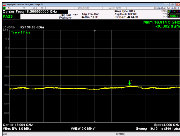
Band 25, LTE10, T, Upper, 14GHz-18GHz
