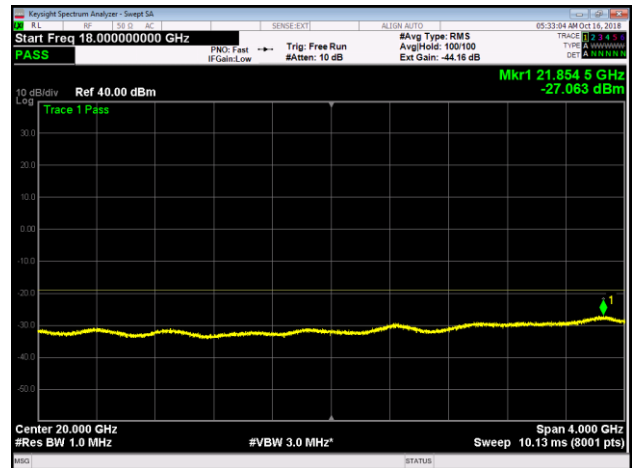
Band 66, LTE10, B, Lower, 18GHz-22GHz
