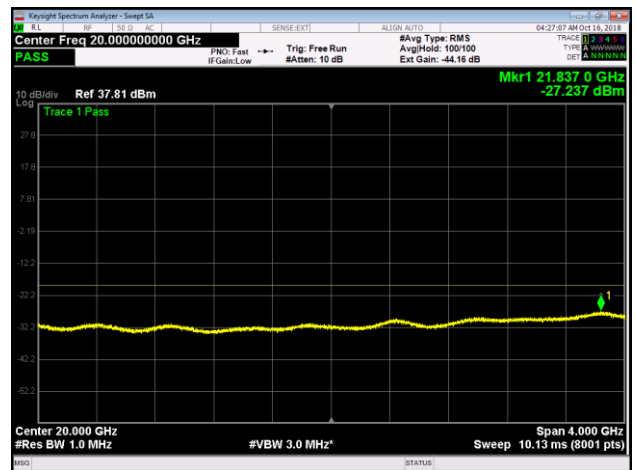
Band 25, LTE10, M, Lower, 18GHz-22GHz
