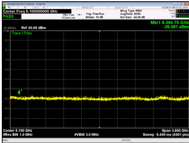
Band 66, LTE10, T, Lower, 6200MHz-10GHz
