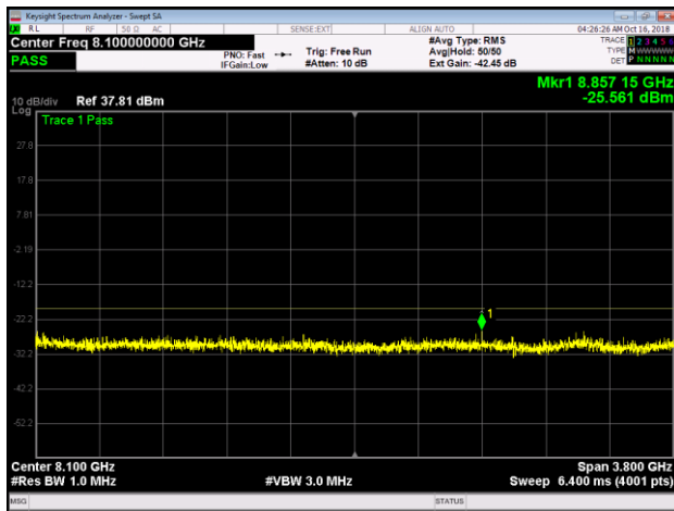
Band 25, LTE10, M, Lower, 6200MHz-10GHz
