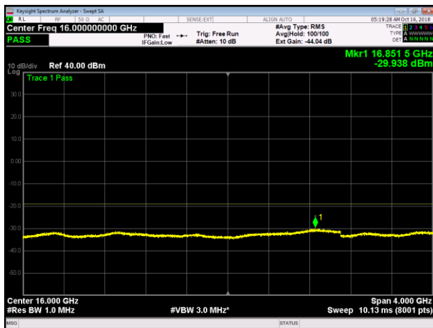
Band 25, LTE10, T, Lower, 14GHz-18GHz
