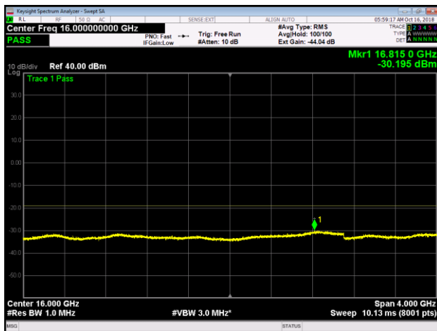
Band 66, LTE10, T, Lower, 14GHz-18GHz
