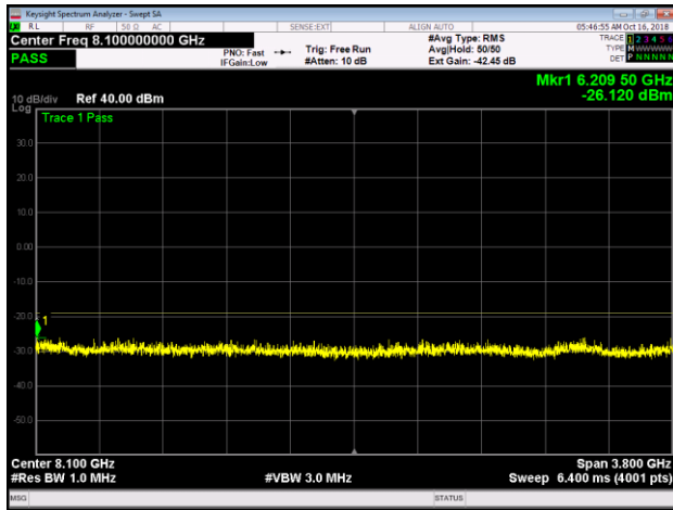
Band 66, LTE10, M, Lower, 6200MHz-10GHz
