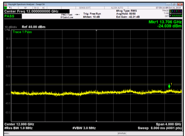
Band 66, LTE10, T, Upper, 10GHz-14GHz
