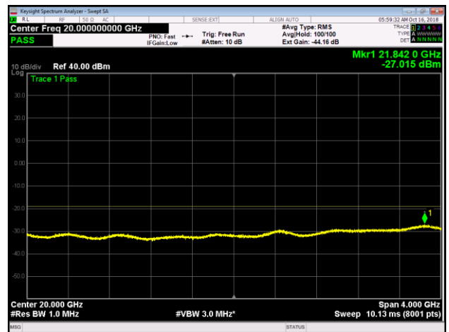
Band 66, LTE10, T, Lower, 18GHz-22GHz
