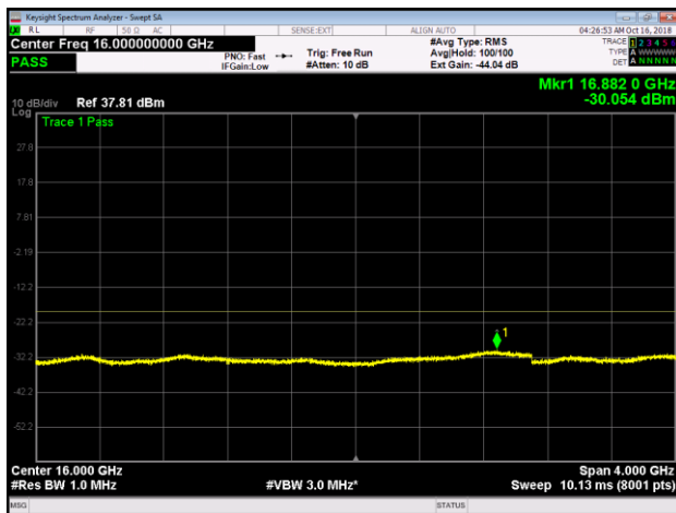
Band 25, LTE10, M, Lower, 14GHz-18GHz
