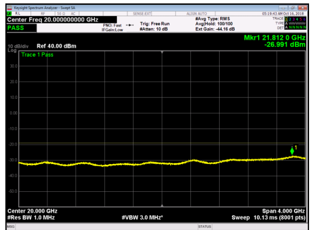
Band 25, LTE10, T, Lower, 18GHz-22GHz
