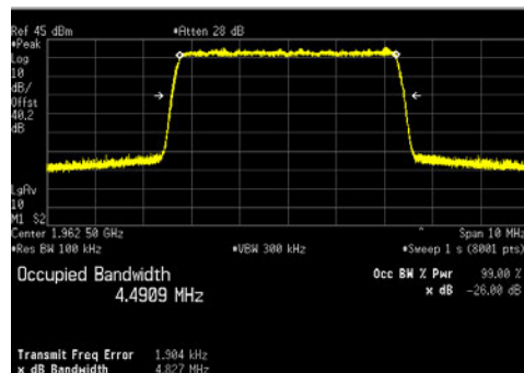
LTE5_64QAM
