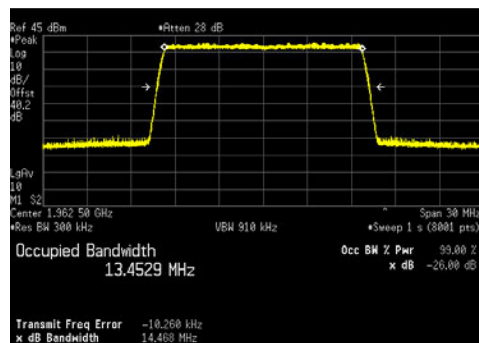
LTE15_64QAM
