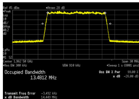
LTE15_16QAM
