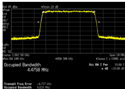
LTE5_16QAM
