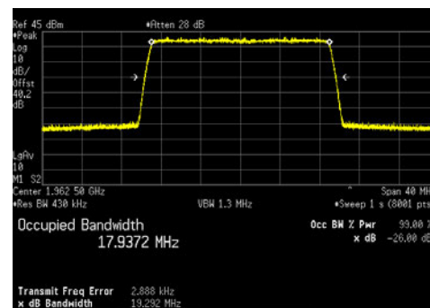
LTE20_64QAM
