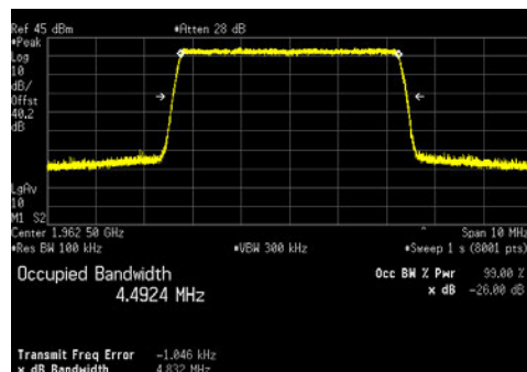
LTE5_256QAM
