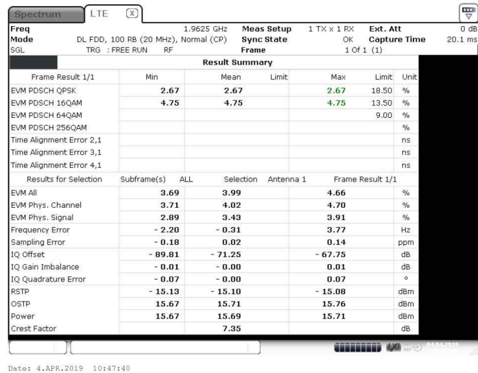
Figure 6 I/Q constellation table with I/Q error – 16QAM (1962.5 MHz) (20MHz Channel BW)
