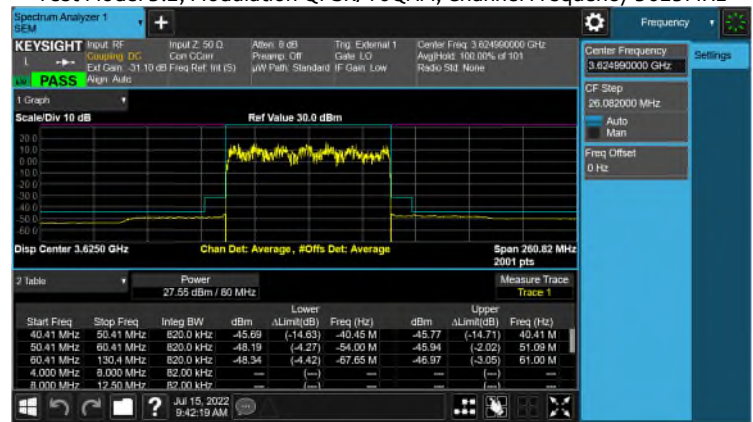
Test Model 3.2, Modulation QPSK/16QAM, Channel Frequency 3625 MHz
