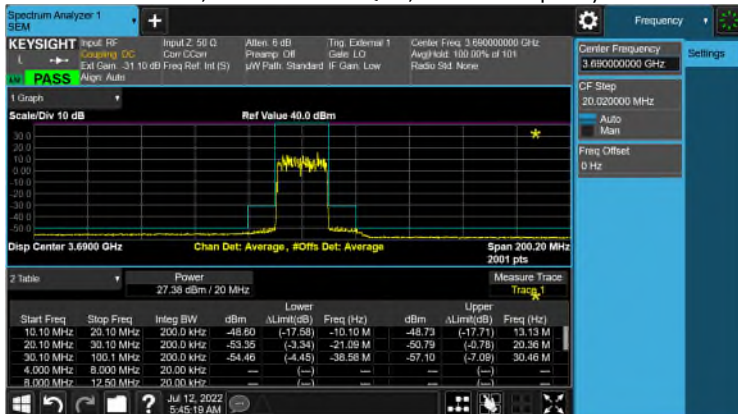
Test Model 3.1a, Modulation 256QAM, Channel Frequency 3690 MHz
