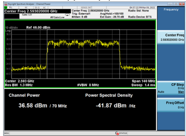
TM3.2, QPSK/16QAM, 2593MHz
