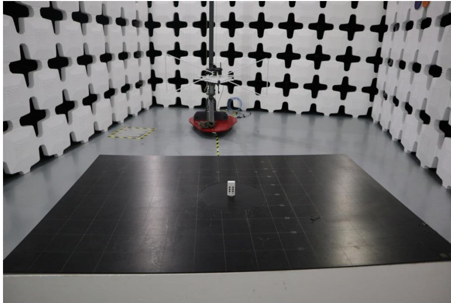
Radiated Spurious Emission 30MHz – 1GHz
