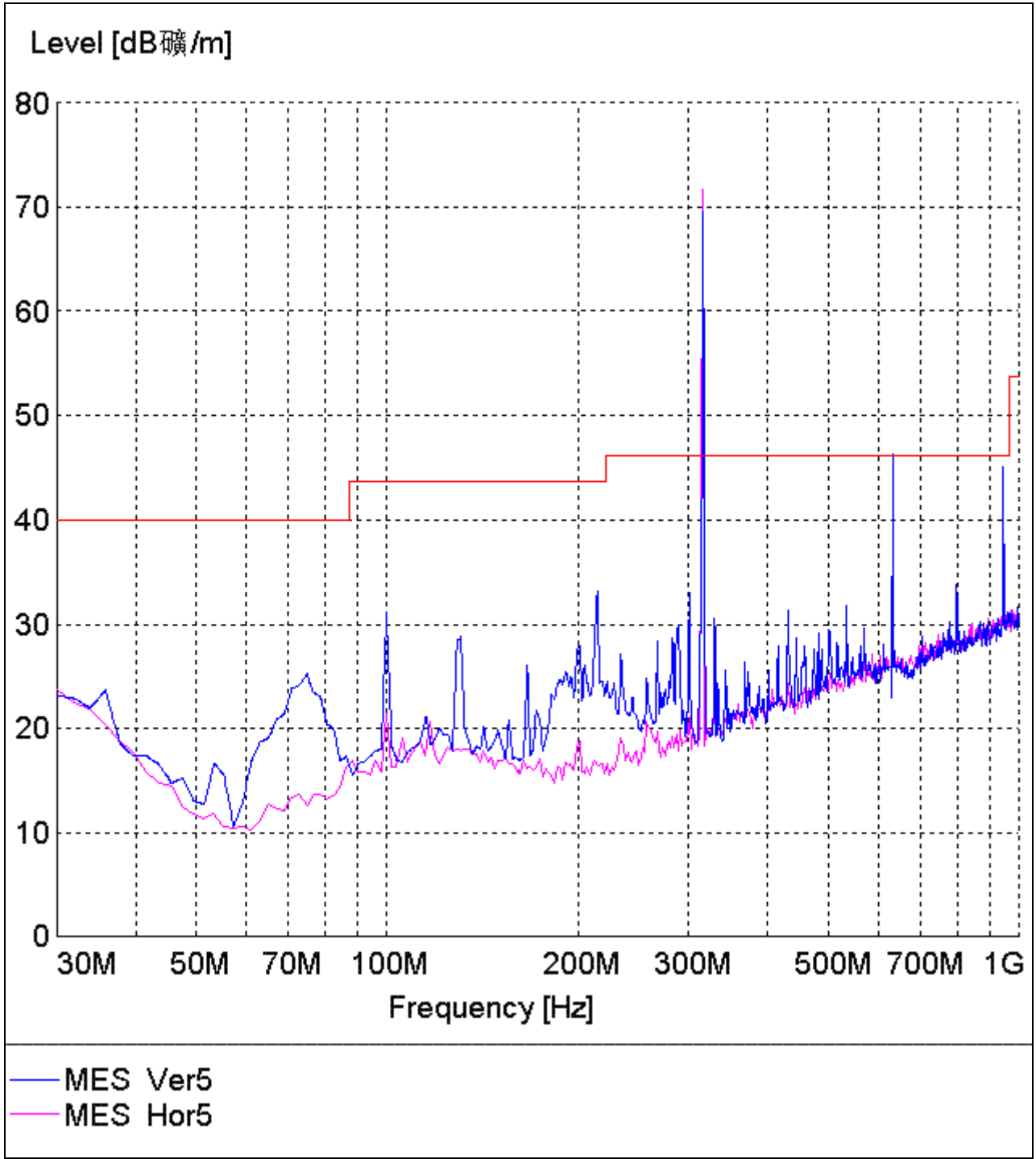
Plot of Radiation Emissions Test (Below 1GHz)
