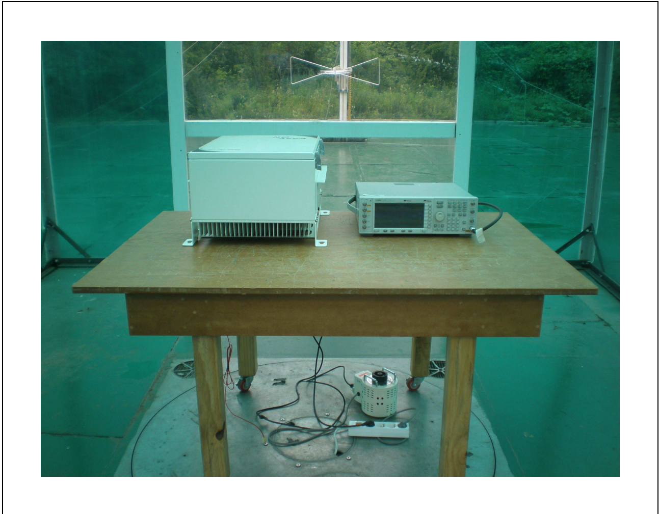
Figure 3 Test setup for Radiated Emissions
