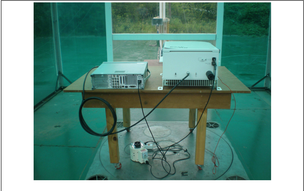
Figure 8 Test setup for Spurious Radiated Emissions
