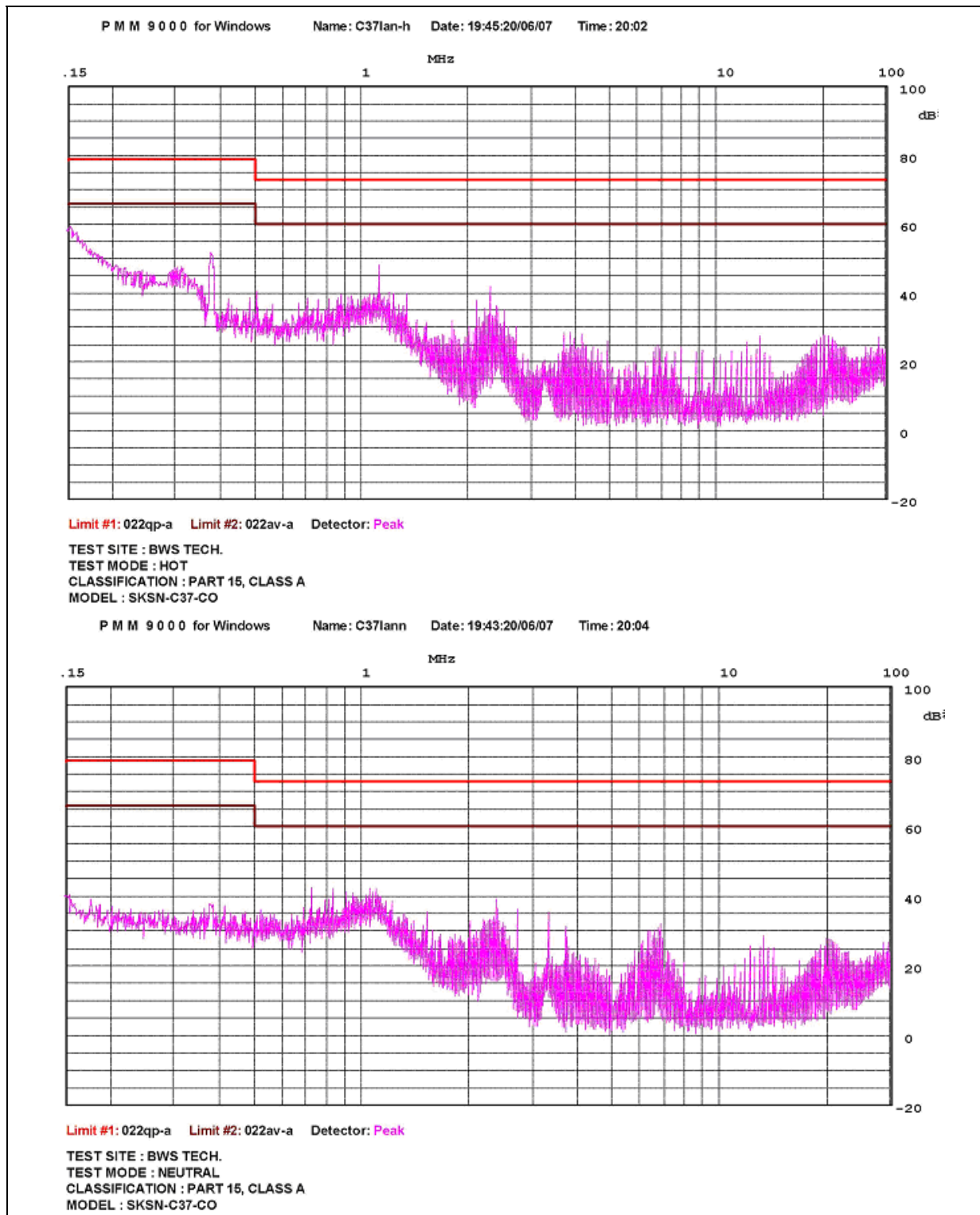
Figure 2 Conducted Emissions Graph – LAN communication mode
