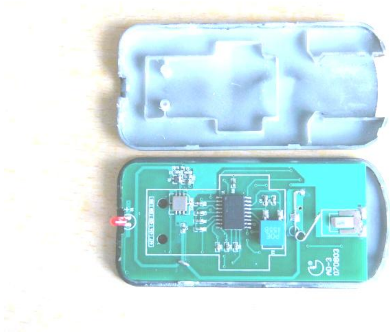
Main board component side
