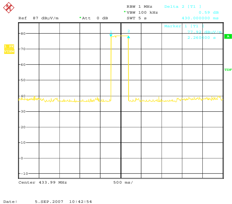
Tranmitter Turn-Off Relaease Time, Upon Momentary Activation of Push Switch (Showing release time less than 1 second)
