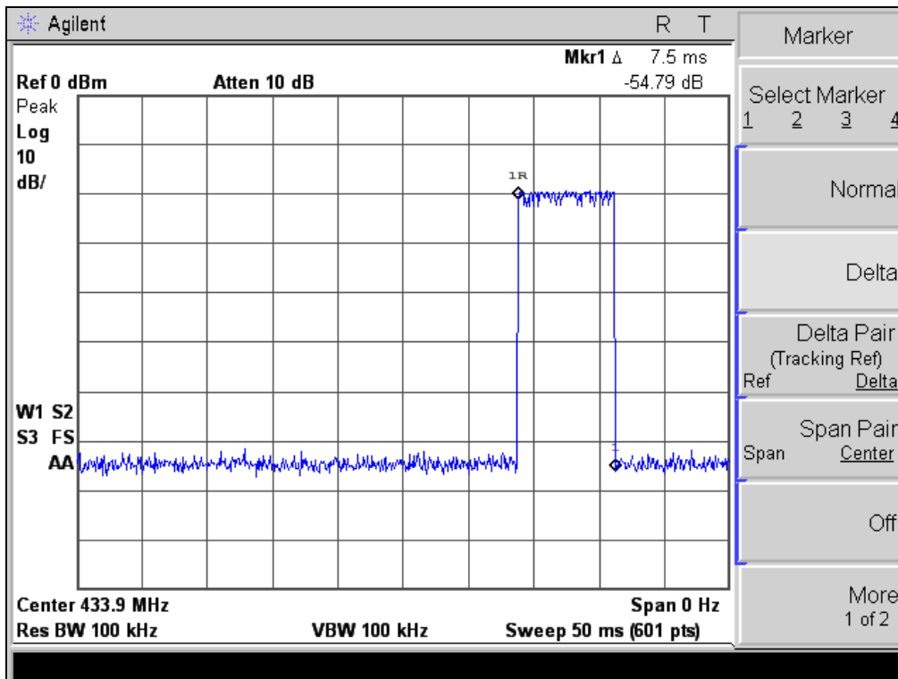
- Transmission Time -
