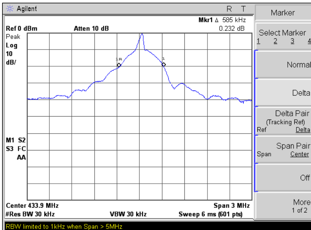
- 20dB Bandwidth -
