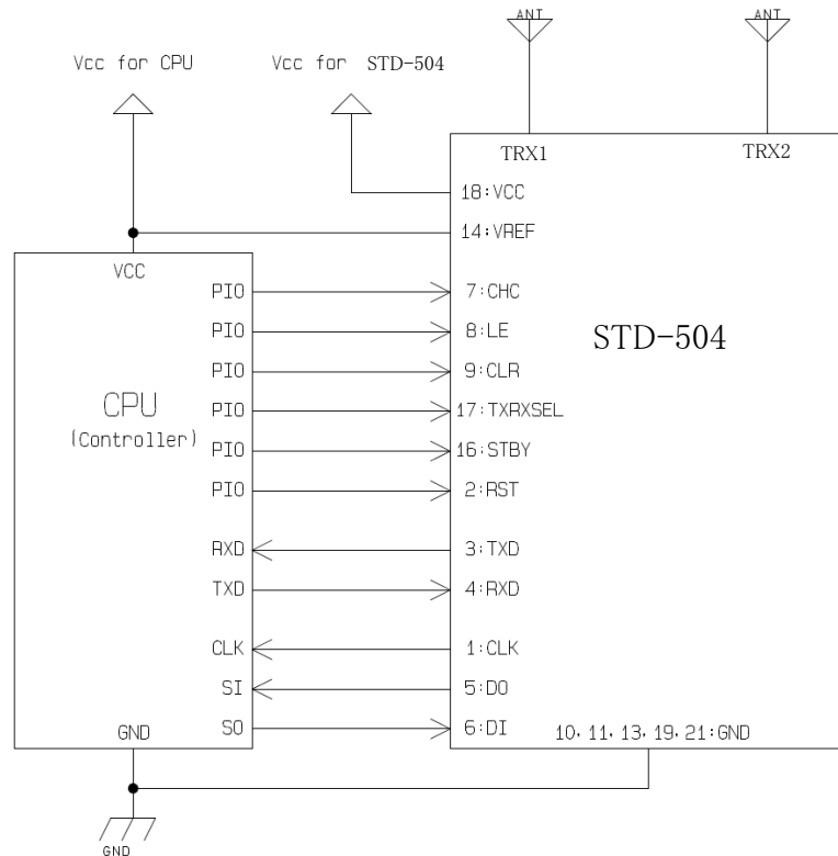
Using a different VCC voltage for the CPU and the STD-504
