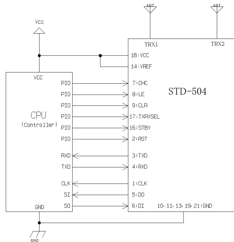
Using a common VCC voltage for the CPU and the STD-504
