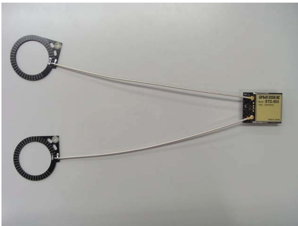
W/Loop PCB antenna
