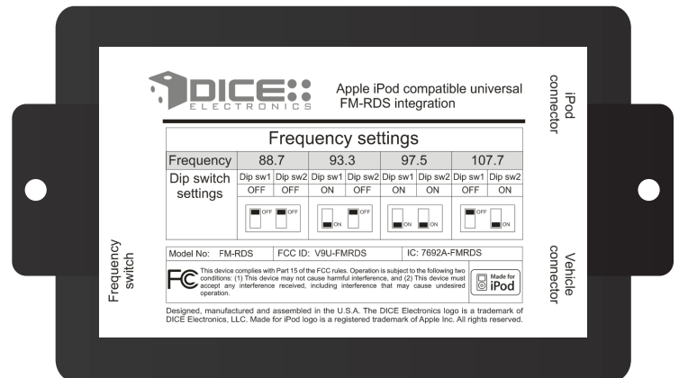
Bottom view of interface module
