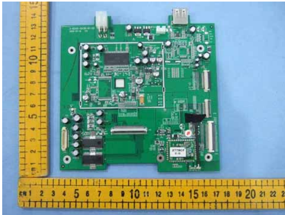
Figure 9 PCB of the EUT Front-View 2
