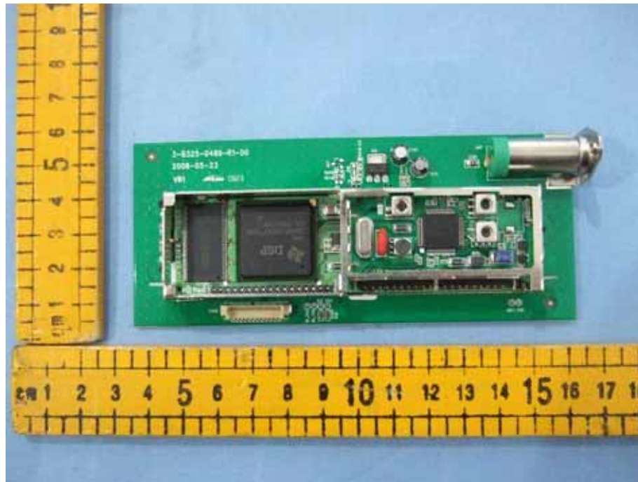
Figure 13 PCB of the EUT Front-View 4
