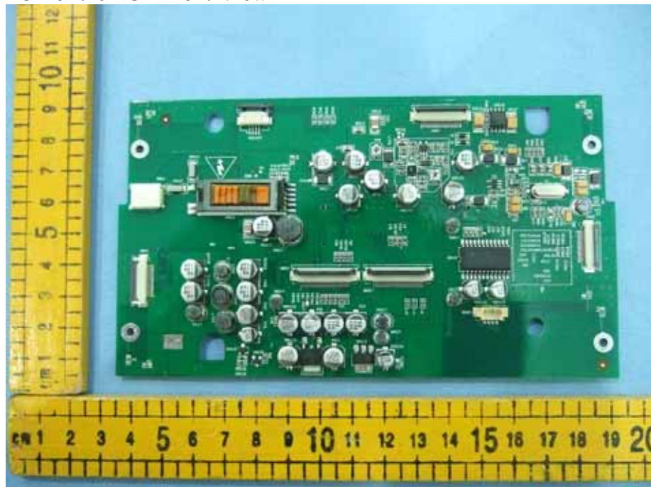
Figure 7 PCB of the EUT Front-View 1
