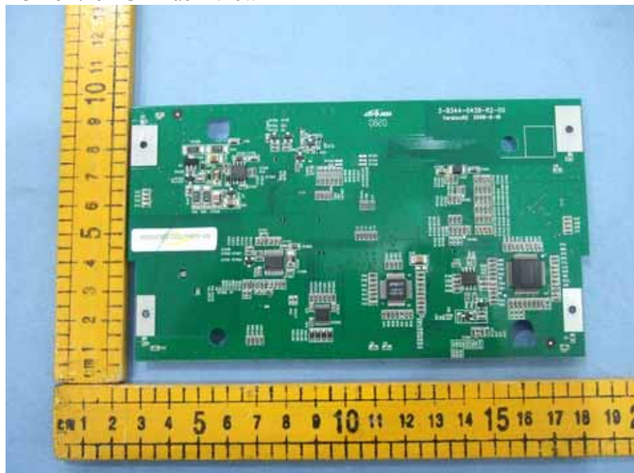
Figure 8 PCB of the EUT Back-View 1
